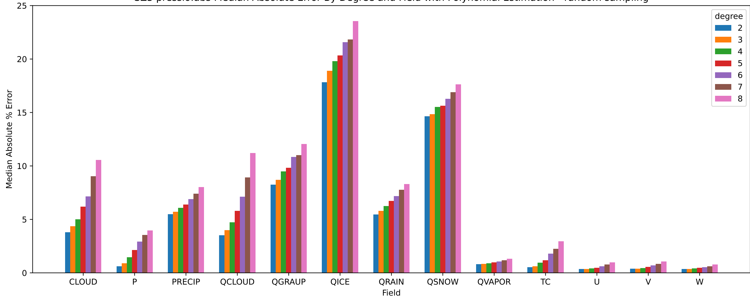
SZ3 pressio:abs Median Absolute Error By Degree and Field with Polynomial Estimation - random sampling
