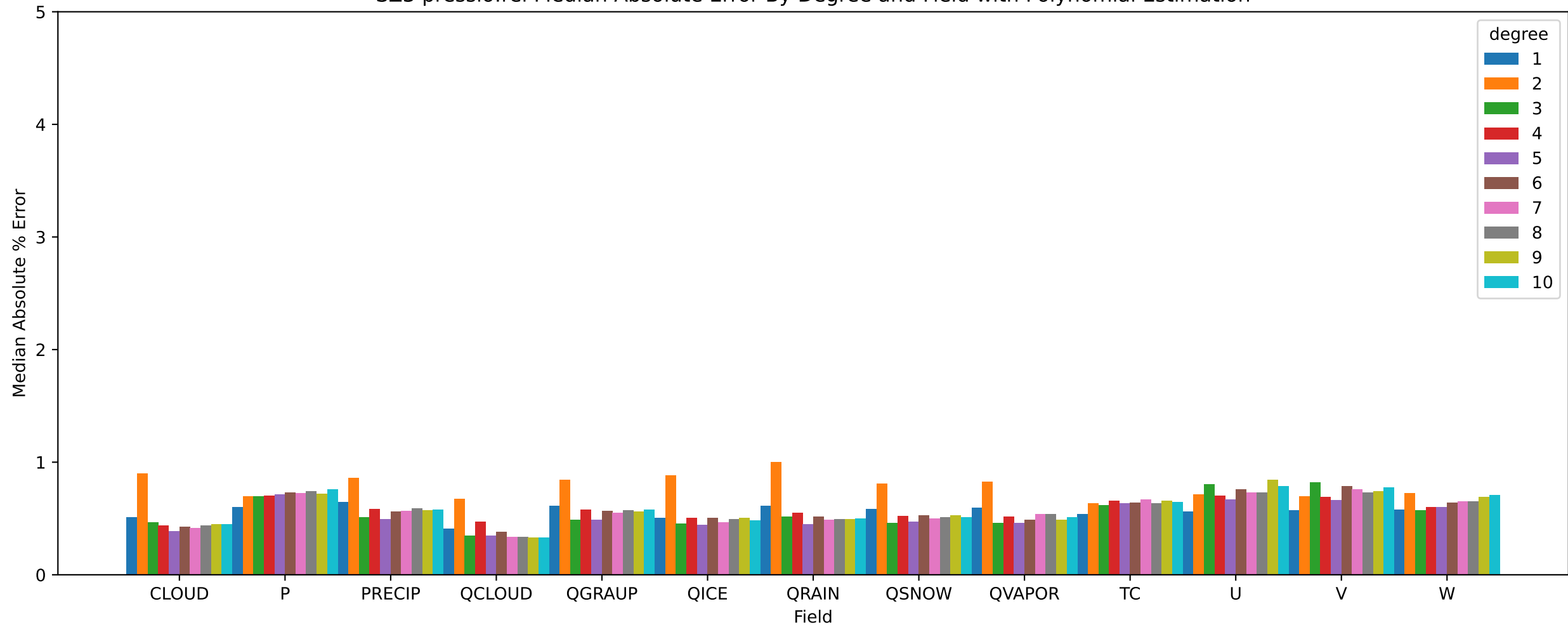
SZ3 pressio:rel Median Absolute Error By Degree and Field with Polynomial Estimation
