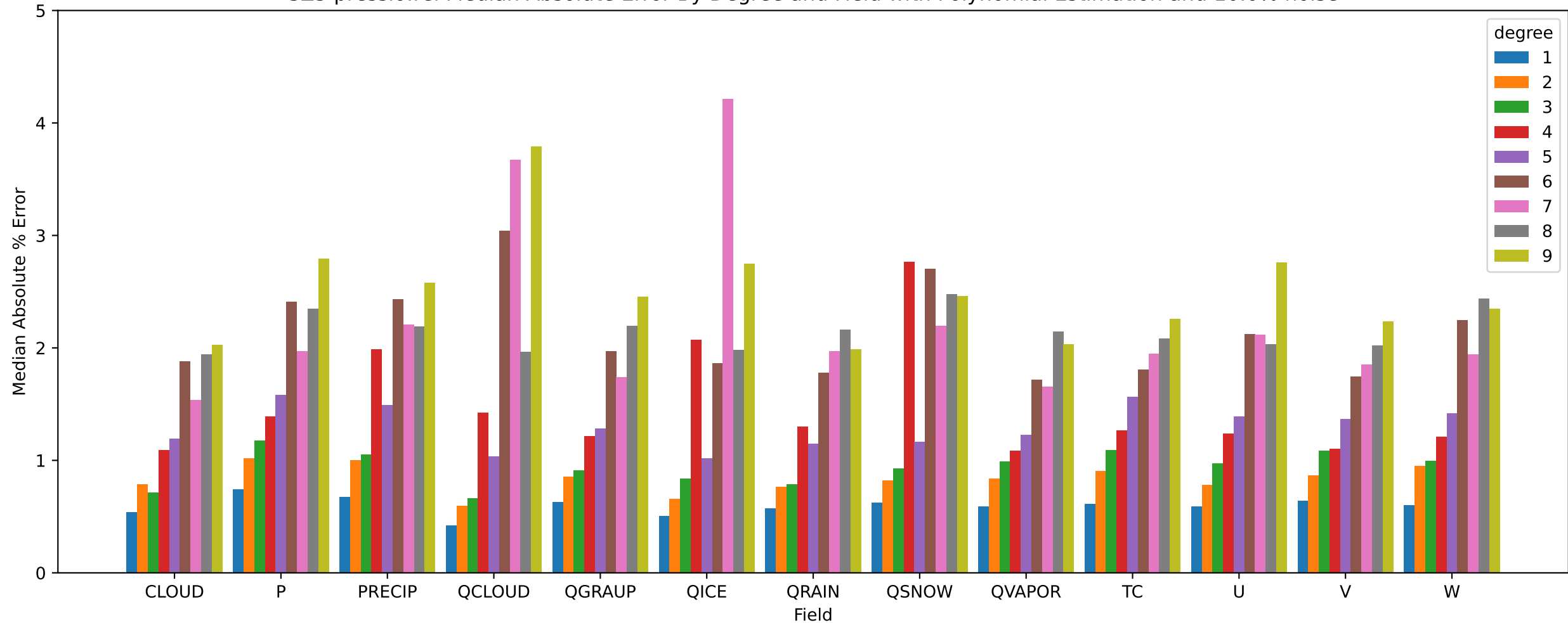
SZ3 pressio:rel Median Absolute Error By Degree and Field with Polynomial Estimation and 10.0% noise
