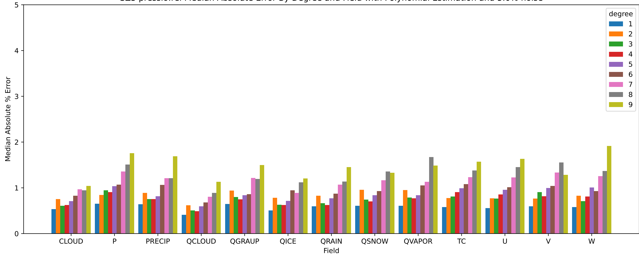
SZ3 pressio:rel Median Absolute Error By Degree and Field with Polynomial Estimation and 5.0% noise
