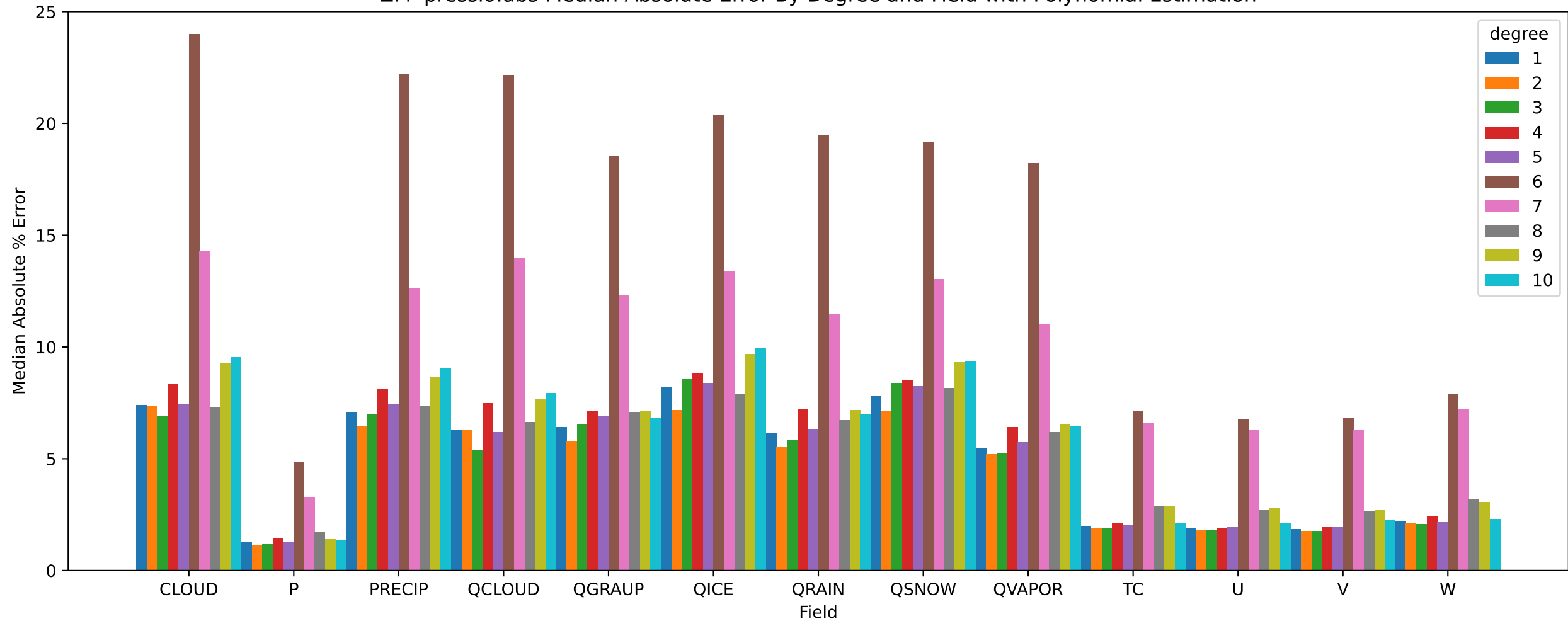
ZFP pressio:abs Median Absolute Error By Degree and Field with Polynomial Estimation
