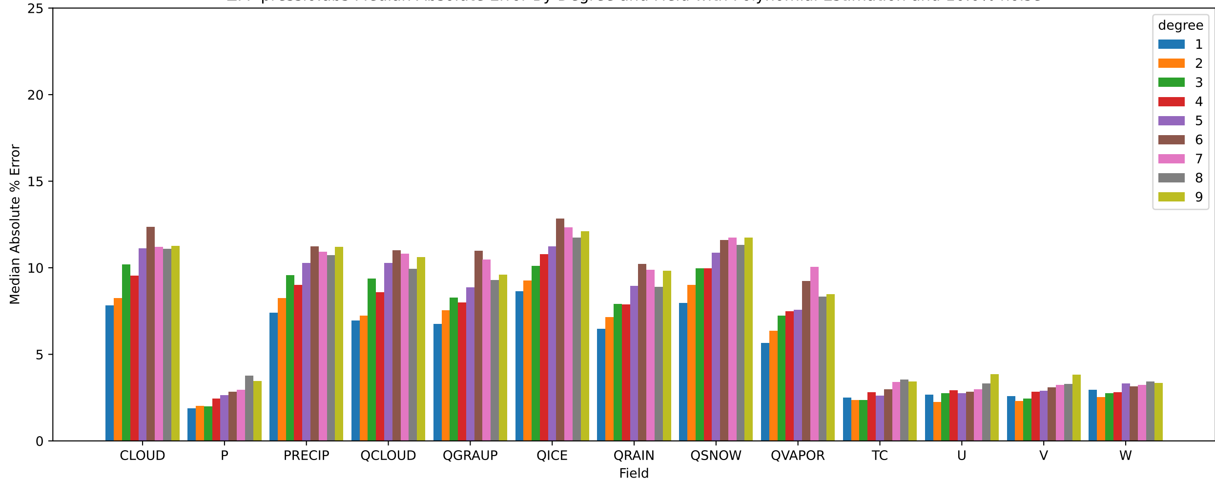
ZFP pressio:abs Median Absolute Error By Degree and Field with Polynomial Estimation and 10.0% noise
