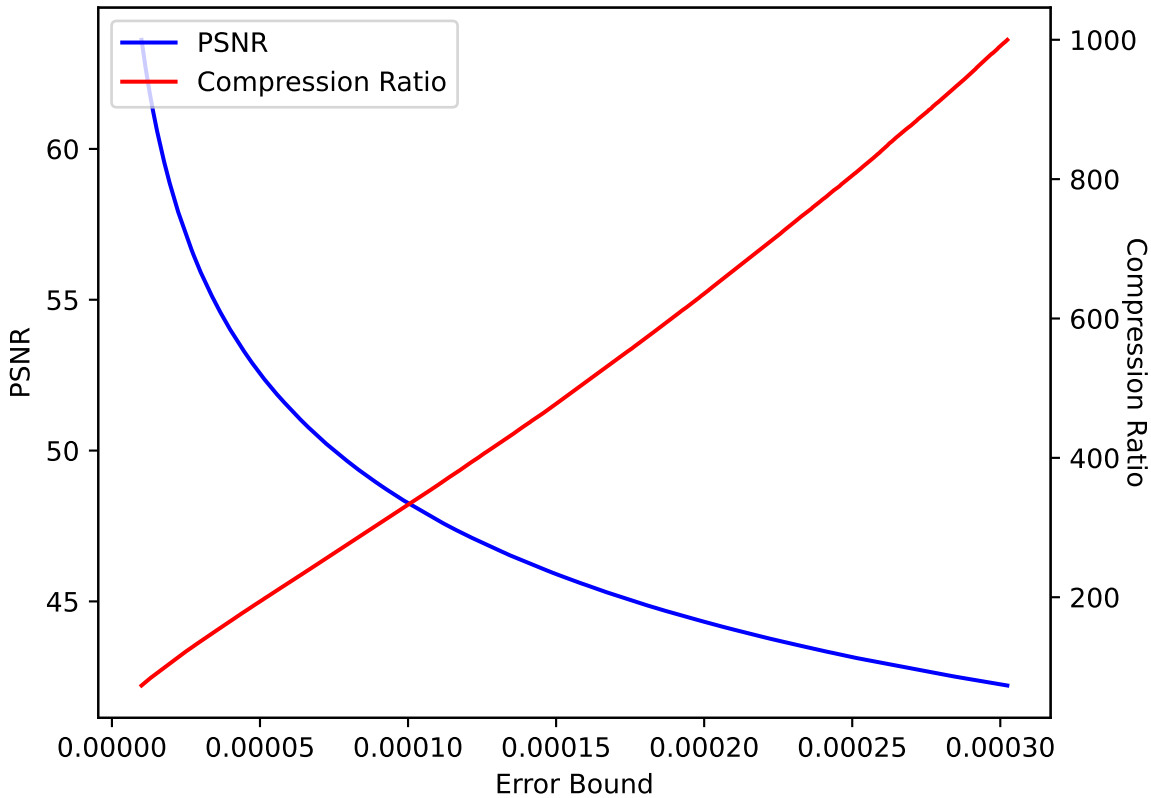
CLOUD 24 SPERR pressio:abs
