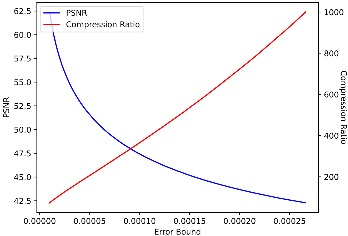
CLOUD 40 SPERR pressio:abs
