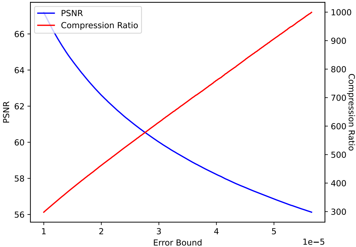
CLOUD 04 SPERR pressio:abs
