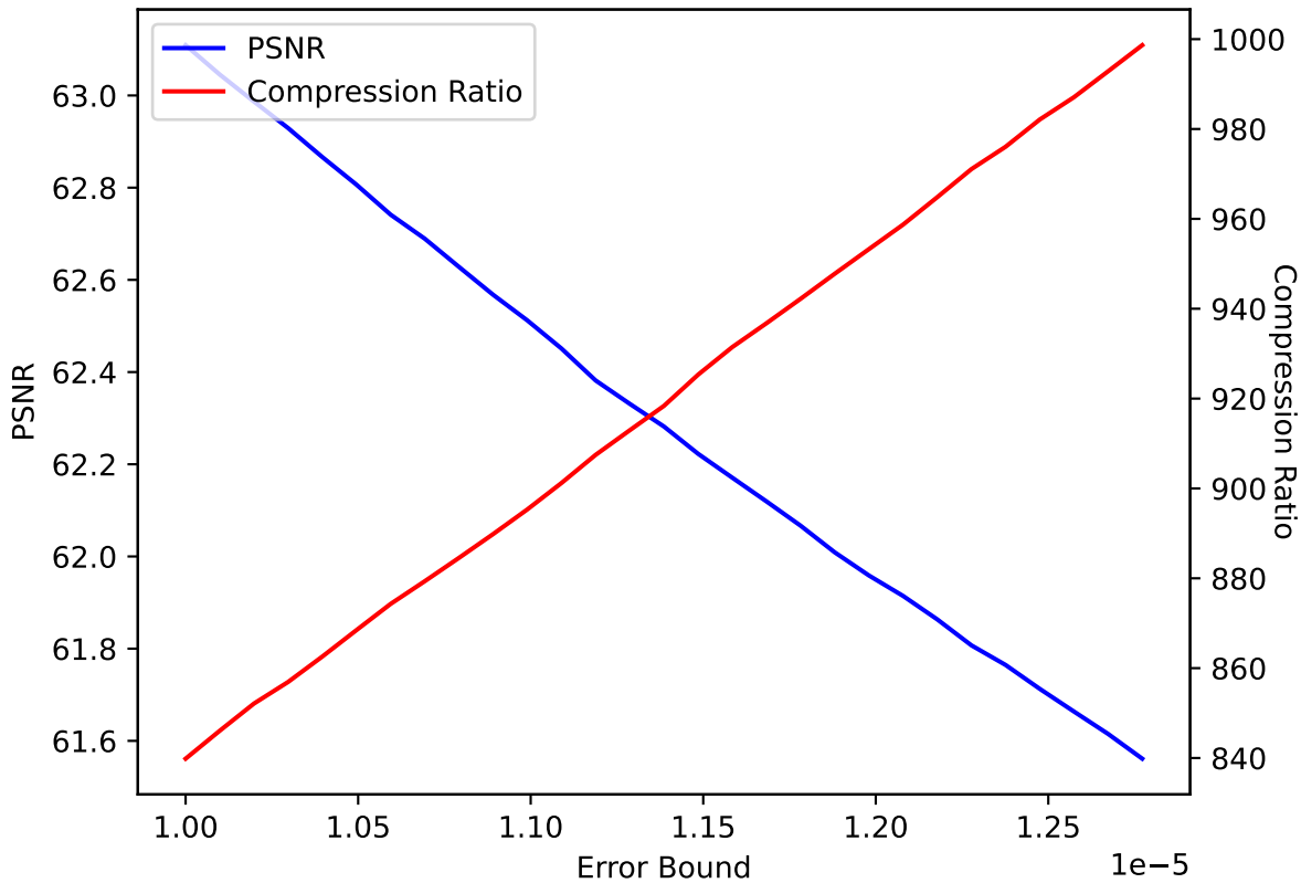
CLOUD 01 SPERR pressio:abs
