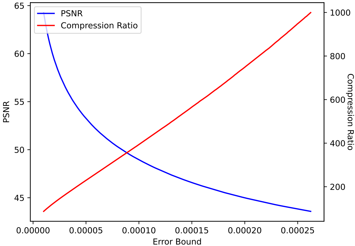
CLOUD 12 SPERR pressio:abs
