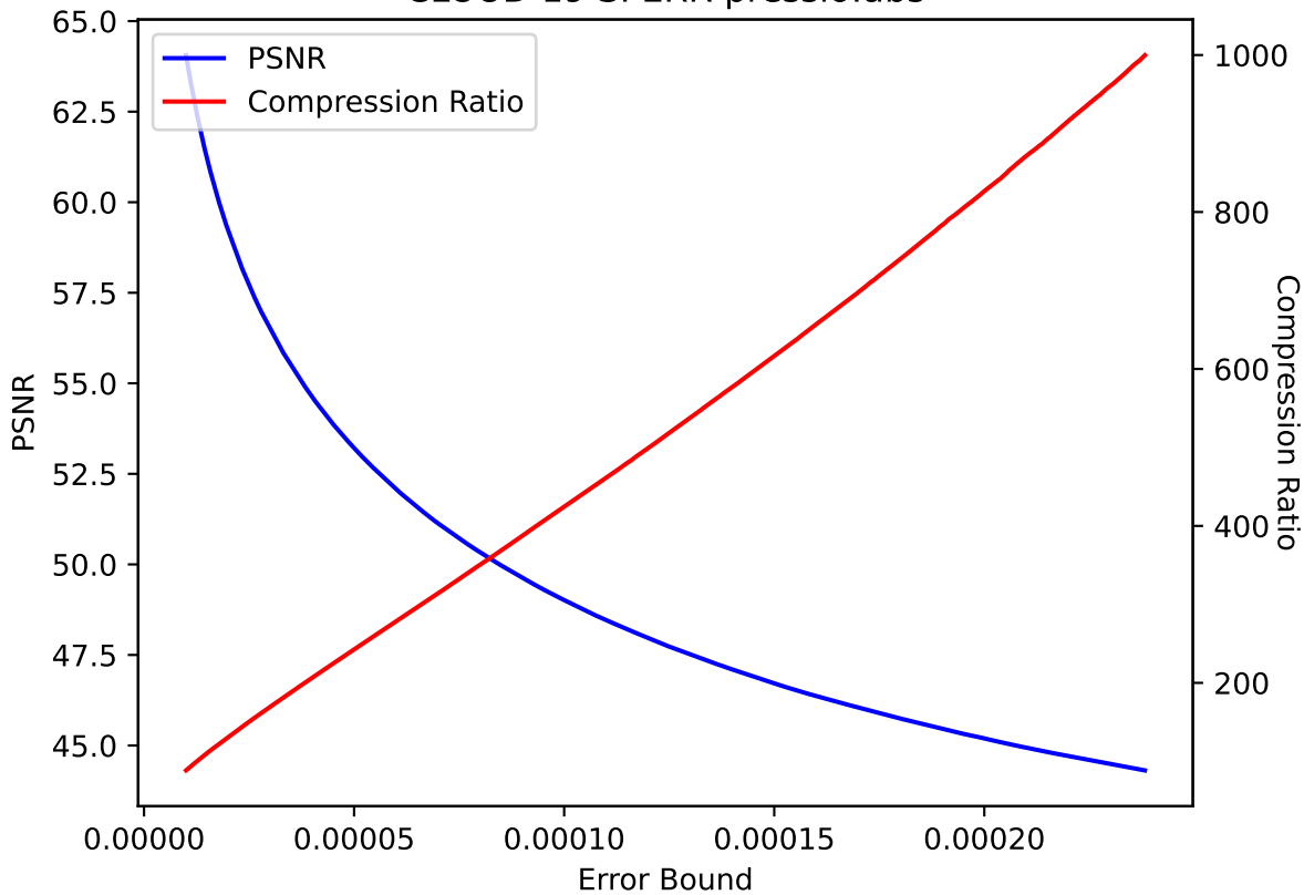
CLOUD 19 SPERR pressio:abs
