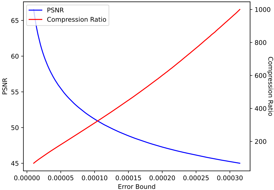
CLOUD 33 SPERR pressio:abs
