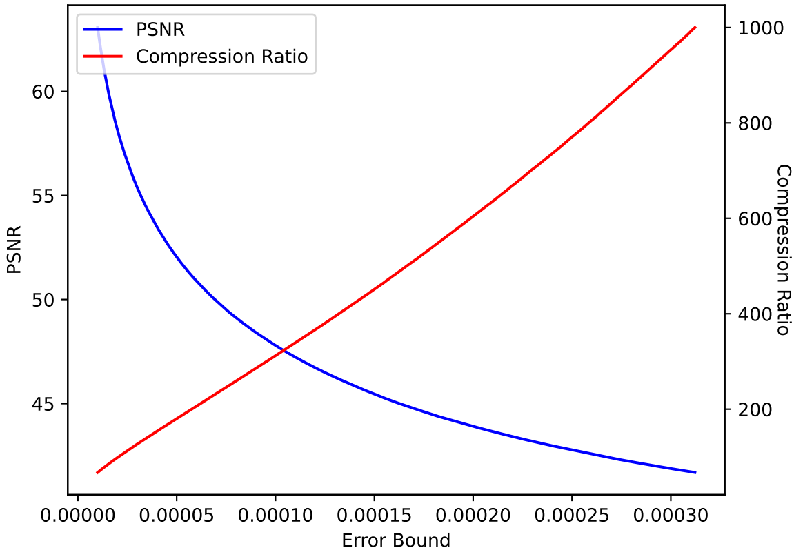
CLOUD 34 SPERR pressio:abs
