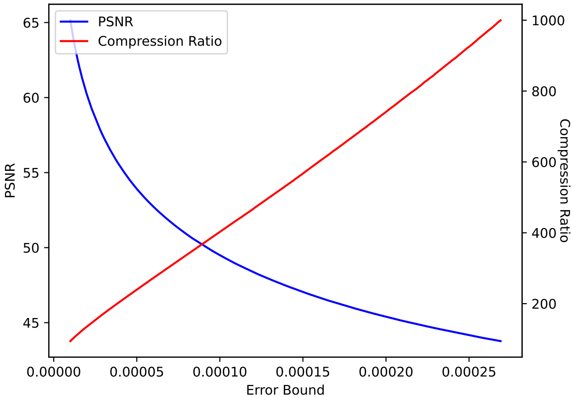
CLOUD 09 SPERR pressio:abs
