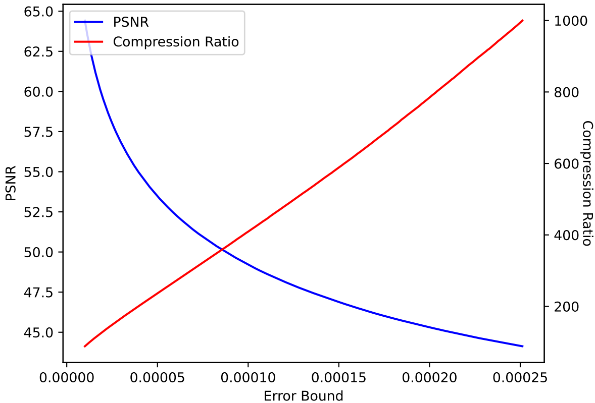
CLOUD 13 SPERR pressio:abs
