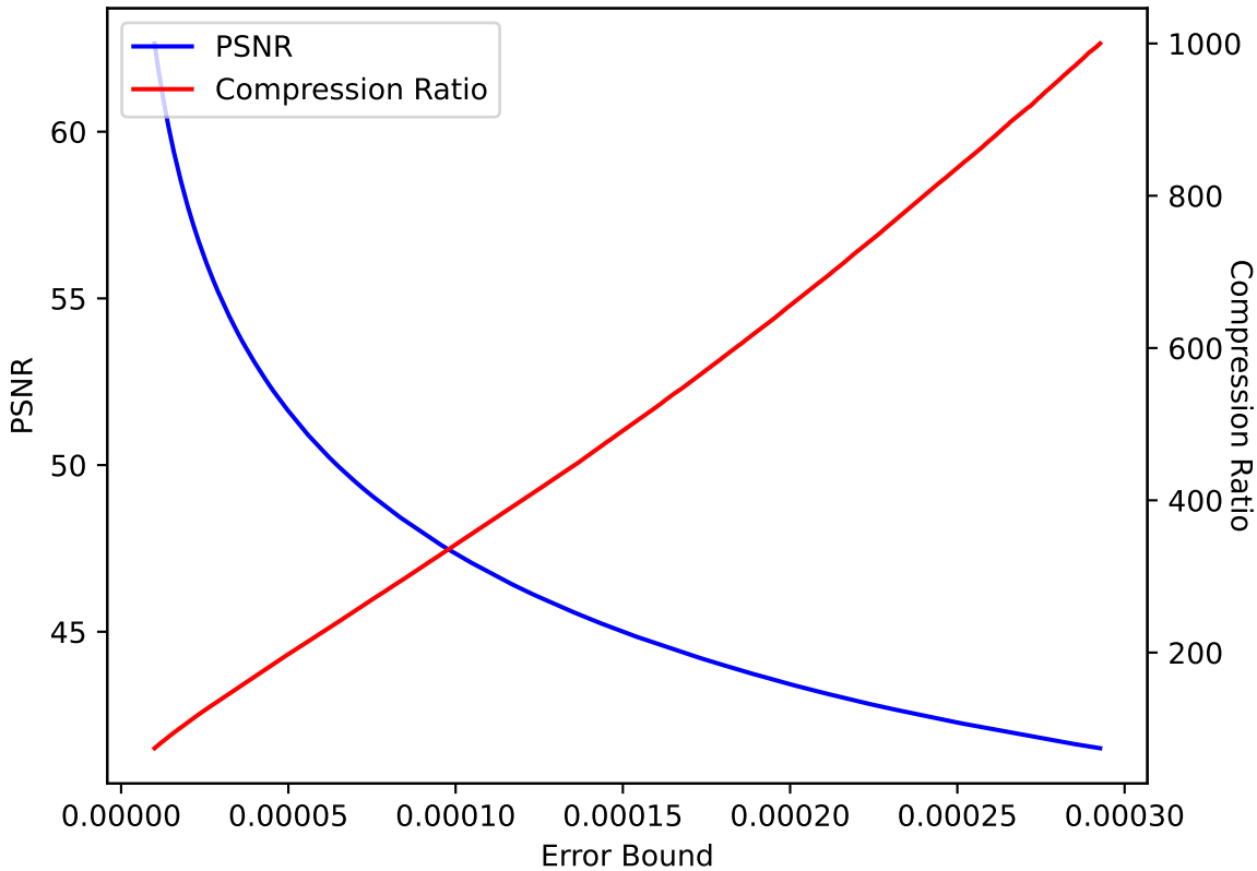
CLOUD 25 SPERR pressio:abs
