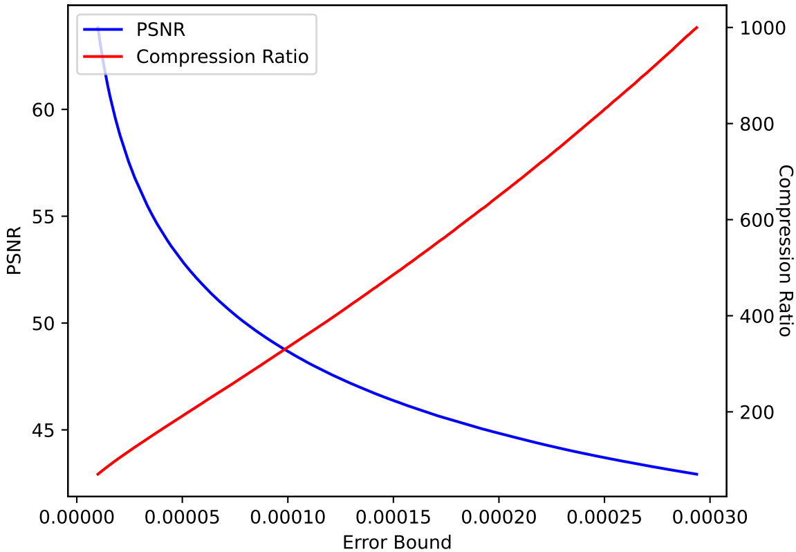
CLOUD 38 SPERR pressio:abs
