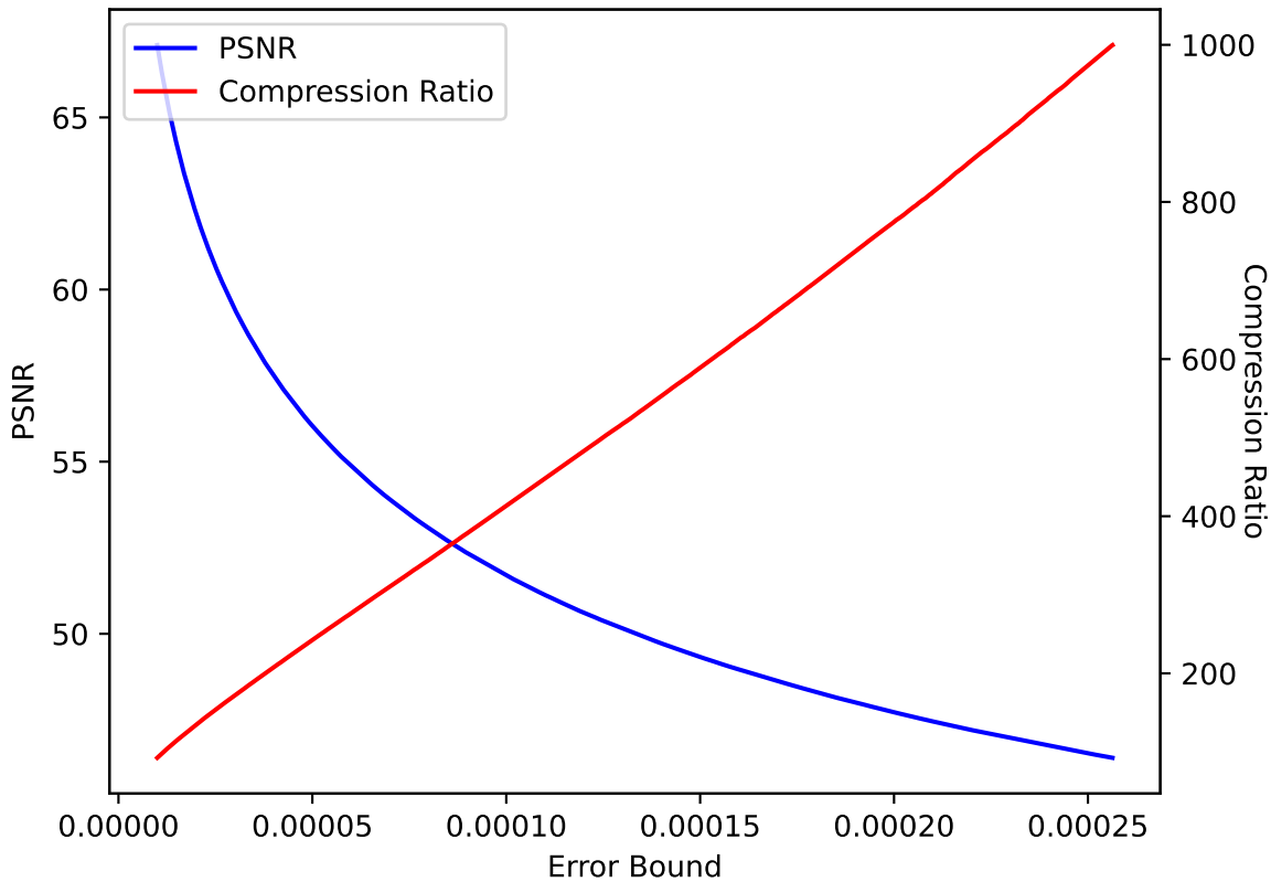
CLOUD 10 SPERR pressio:abs
