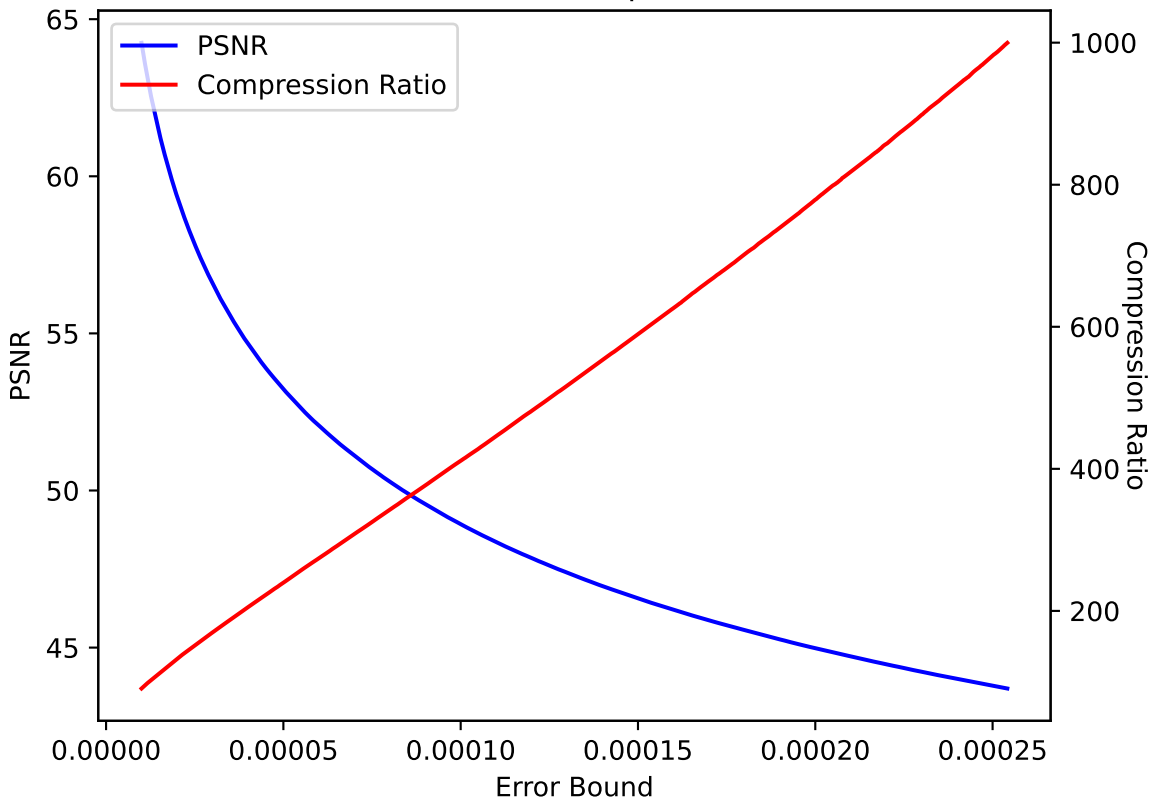
CLOUD 11 SPERR pressio:abs
