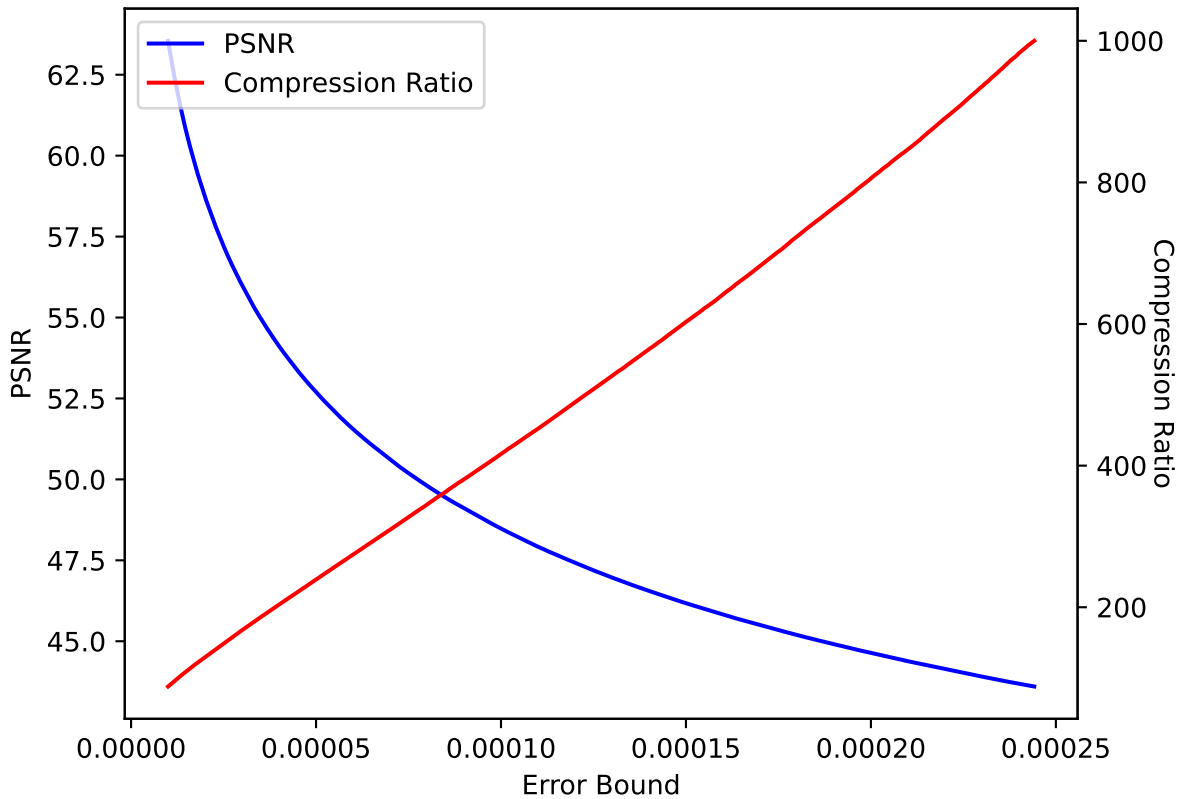
CLOUD 15 SPERR pressio:abs
