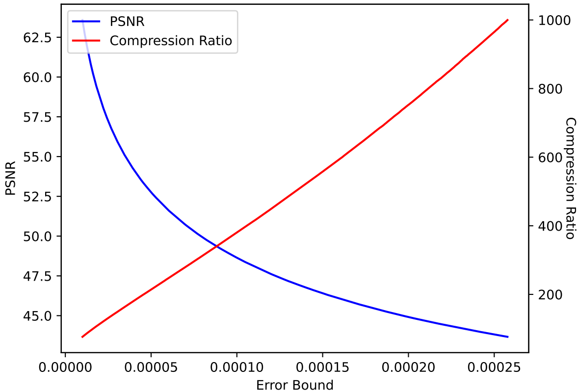
CLOUD 45 SPERR pressio:abs
