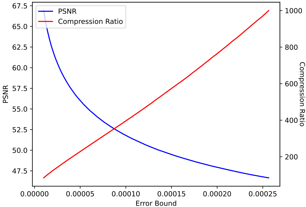
CLOUD 20 SPERR pressio:abs
