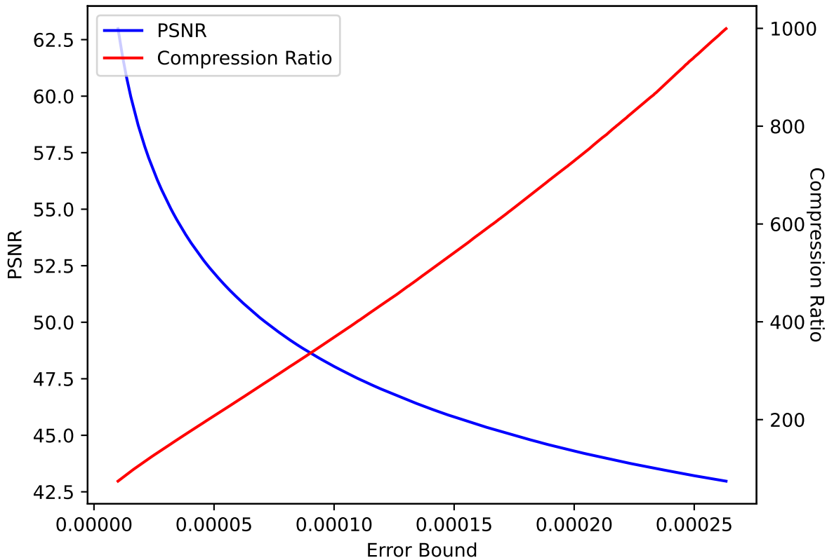
CLOUD 42 SPERR pressio:abs
