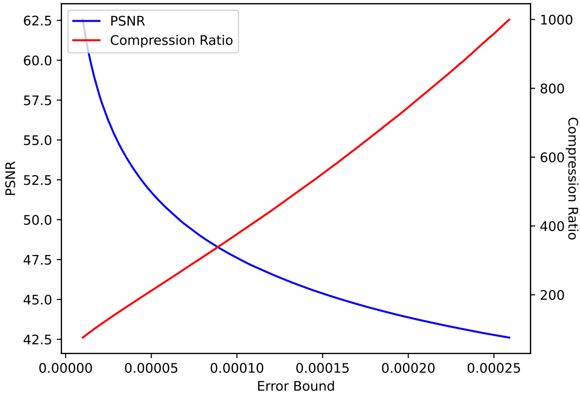
CLOUD 43 SPERR pressio:abs
