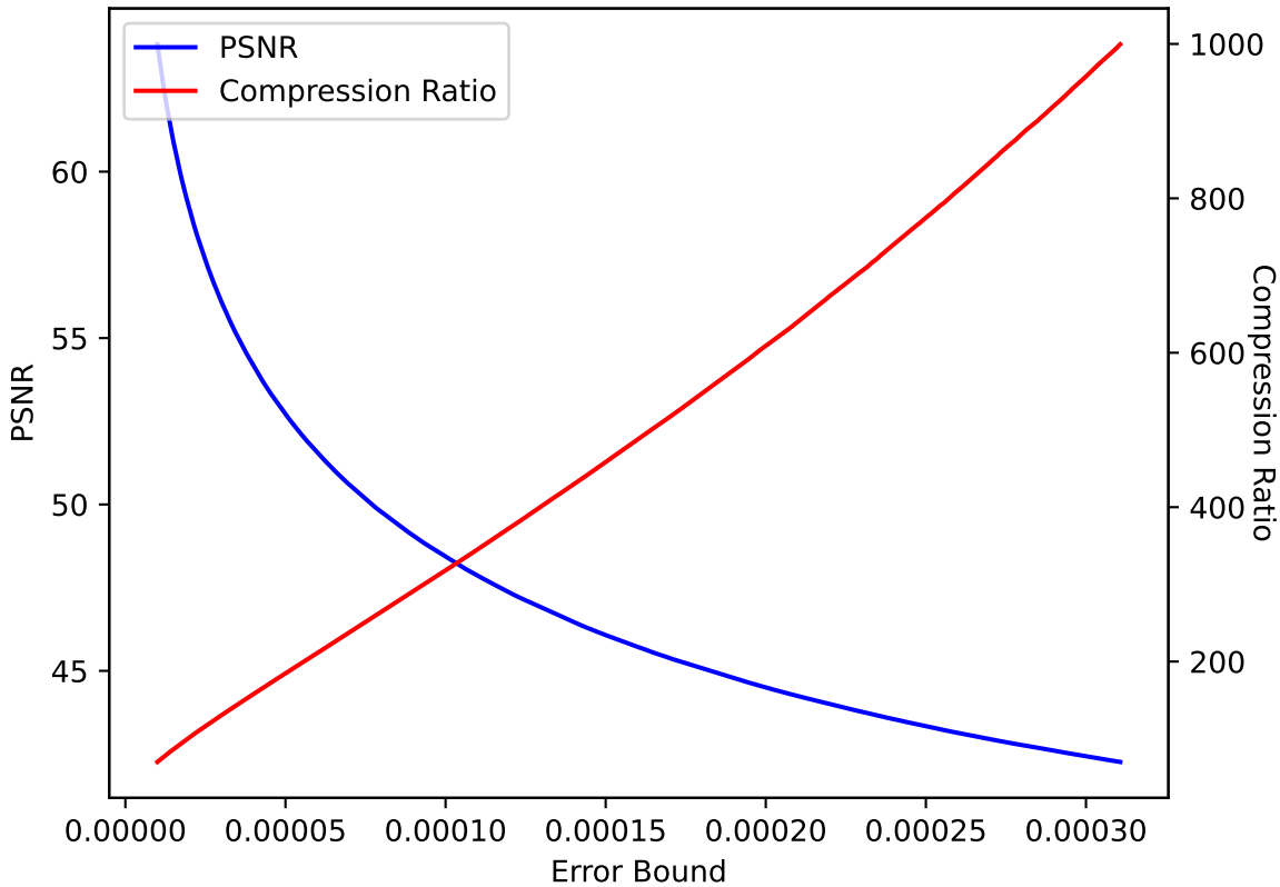
CLOUD 30 SPERR pressio:abs
