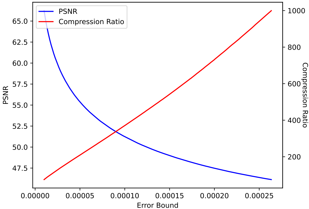
CLOUD 46 SPERR pressio:abs
