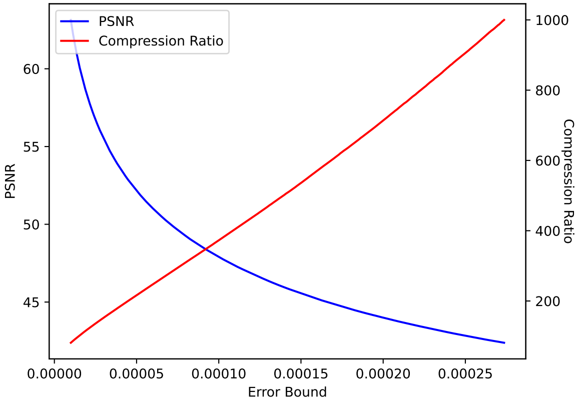
CLOUD 21 SPERR pressio:abs
