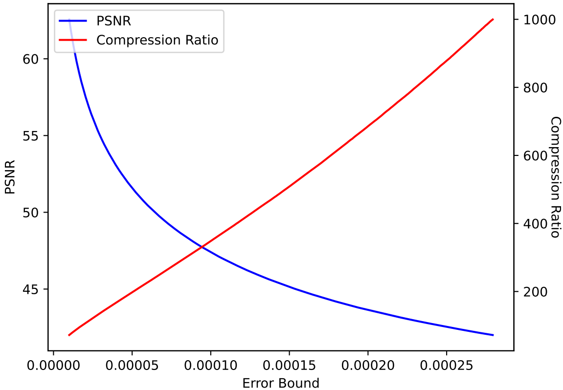
CLOUD 48 SPERR pressio:abs
