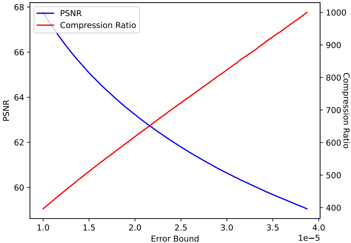
CLOUD 03 SPERR pressio:abs
