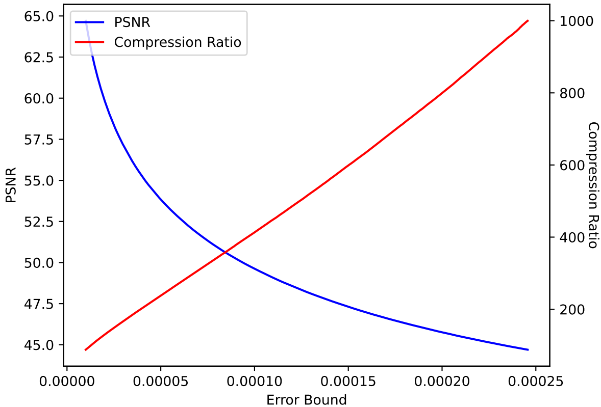
CLOUD 14 SPERR pressio:abs
