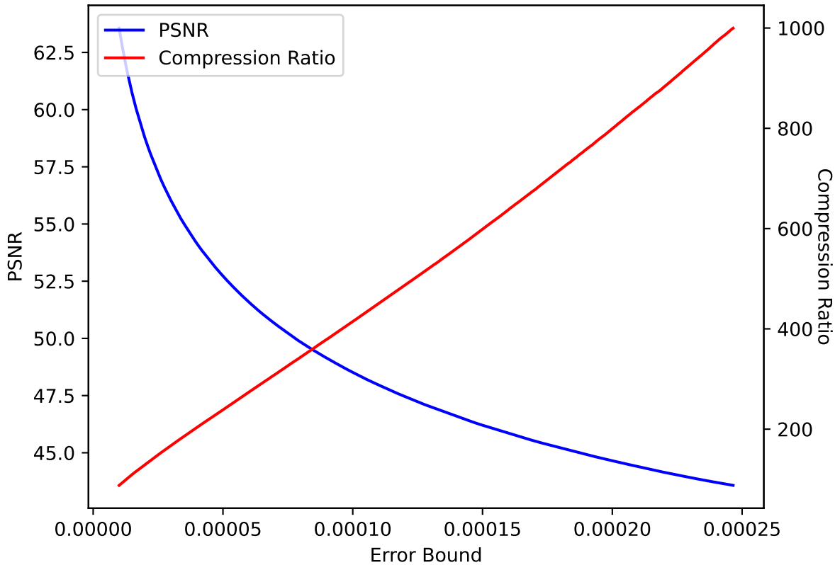
CLOUD 16 SPERR pressio:abs
