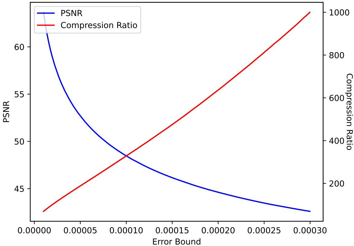
CLOUD 37 SPERR pressio:abs
