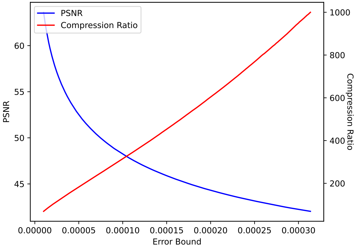
CLOUD 31 SPERR pressio:abs
