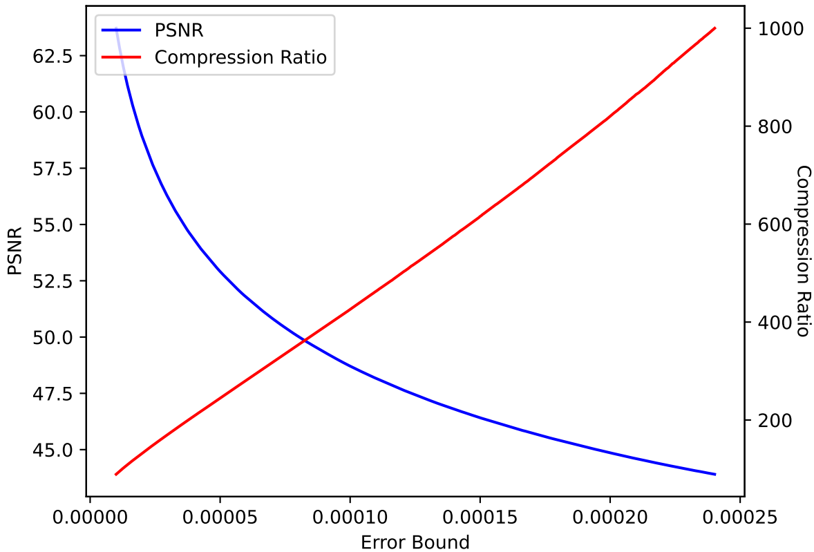
CLOUD 17 SPERR pressio:abs
