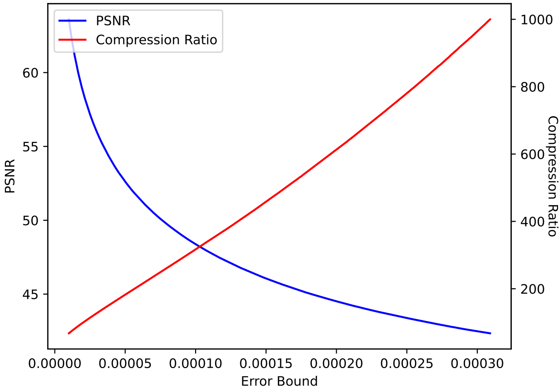
CLOUD 36 SPERR pressio:abs
