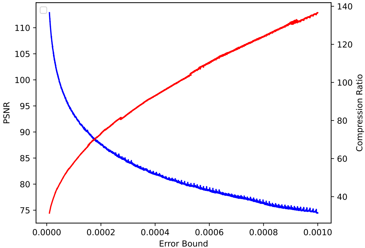
CLOUD 05 pressio:rel
