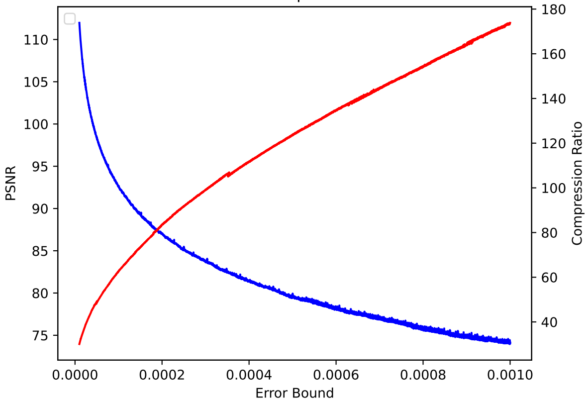
CLOUD 03 pressio:rel
