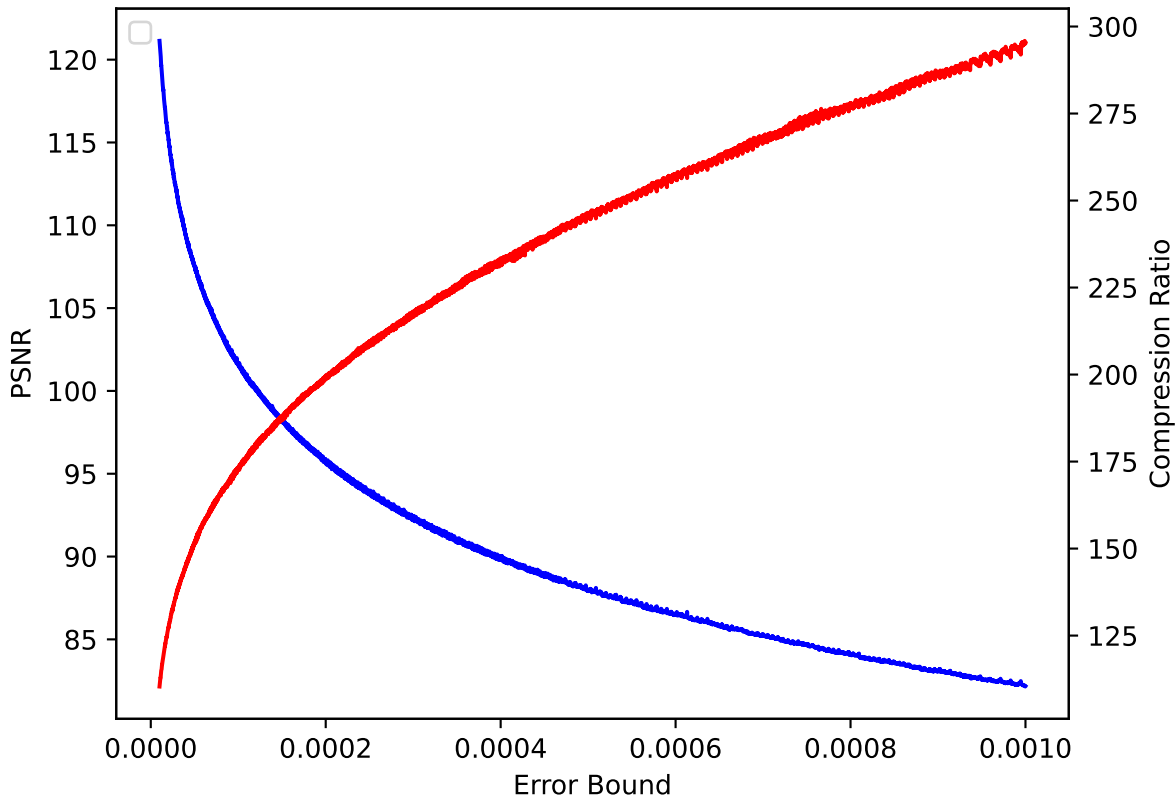
QCLLOUD 05 pressio:rel
