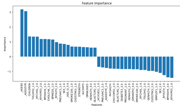
Figure 2: Features
