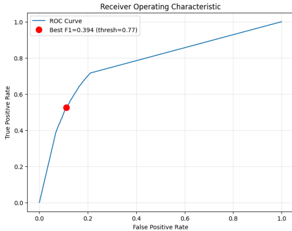
Figure 1: ROC Curve
