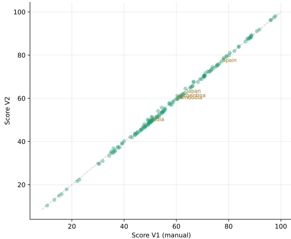
V1 vs V2 (Ridge) — r=0.9995
