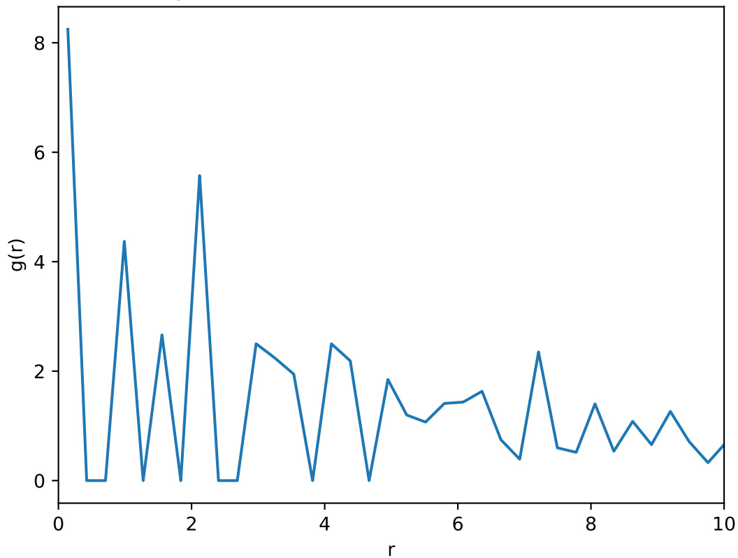
Average radial distribution function: T=0.30 , L=20
