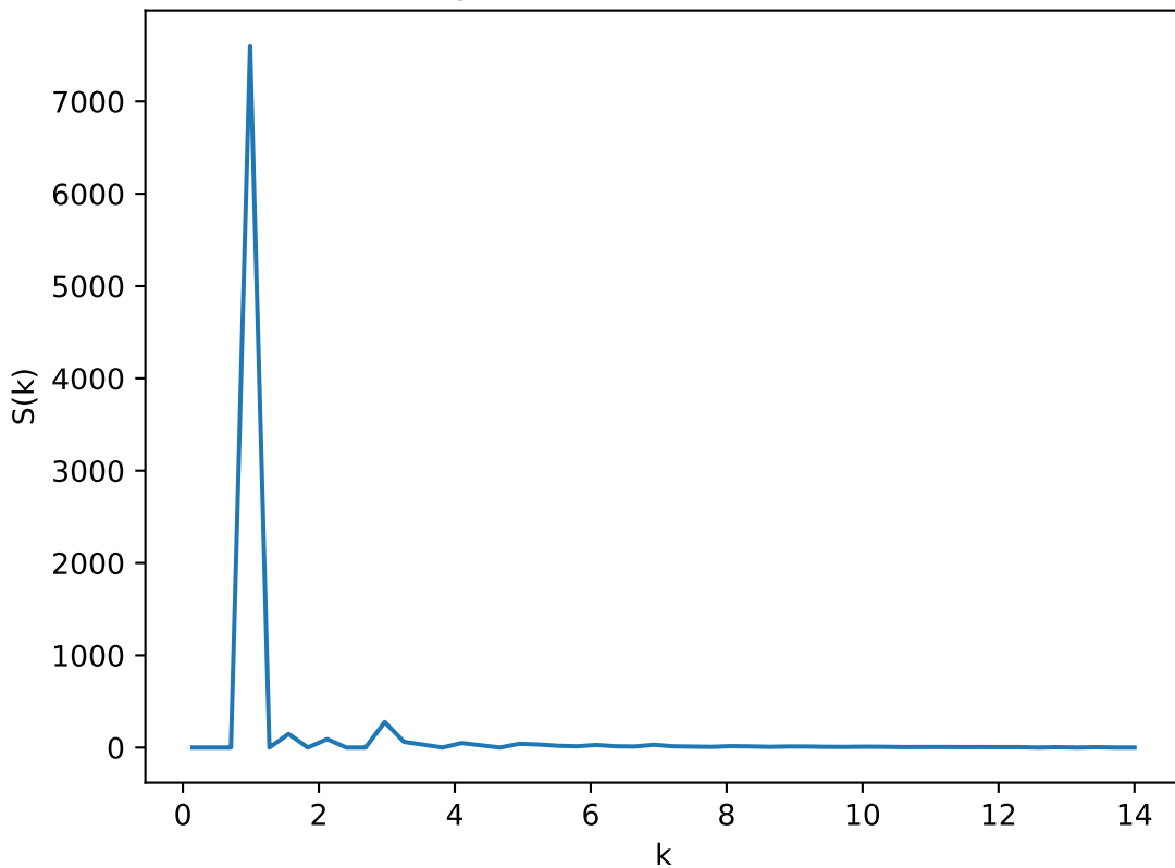
Radial Average of Structure Factor: T=0.30 , L=20
