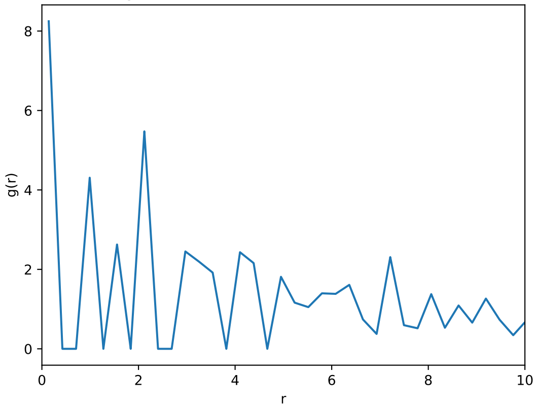
Average radial distribution function: T=0.35 , L=20
