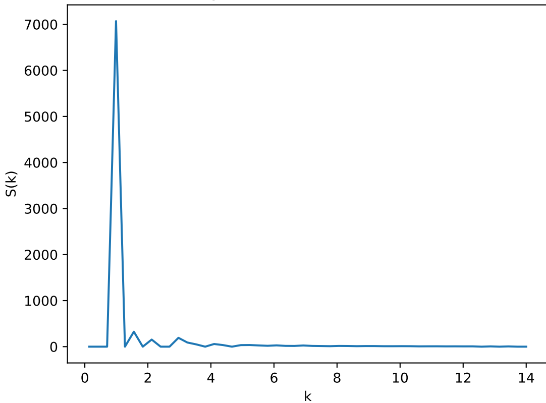
Radial Average of Structure Factor: T=0.35 , L=20
