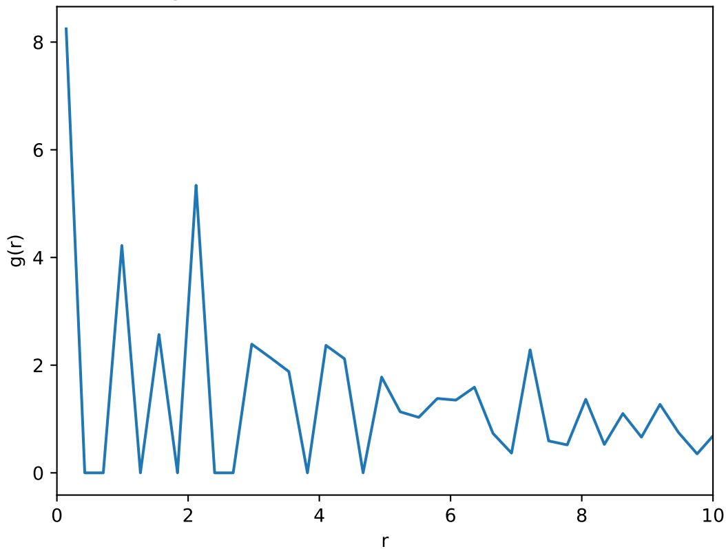
Average radial distribution function: T=0.41 , L=20
