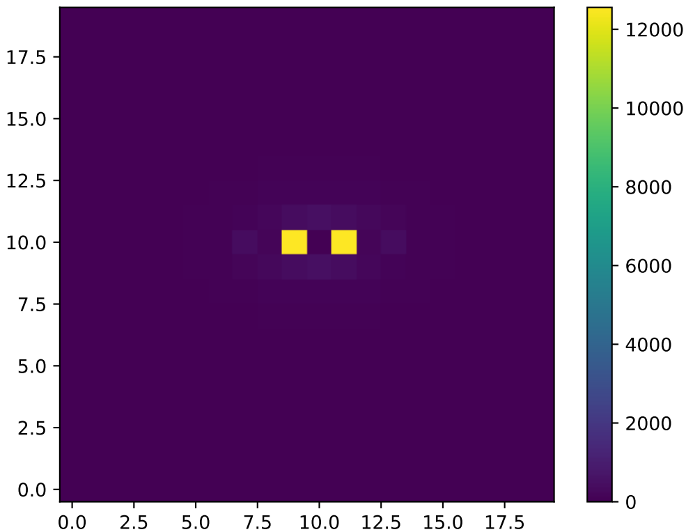
2D Structure Factor S(k) : T=0.41 , L=20
