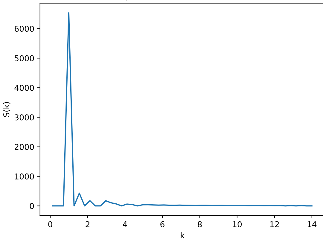
Radial Average of Structure Factor: T=0.41 , L=20
