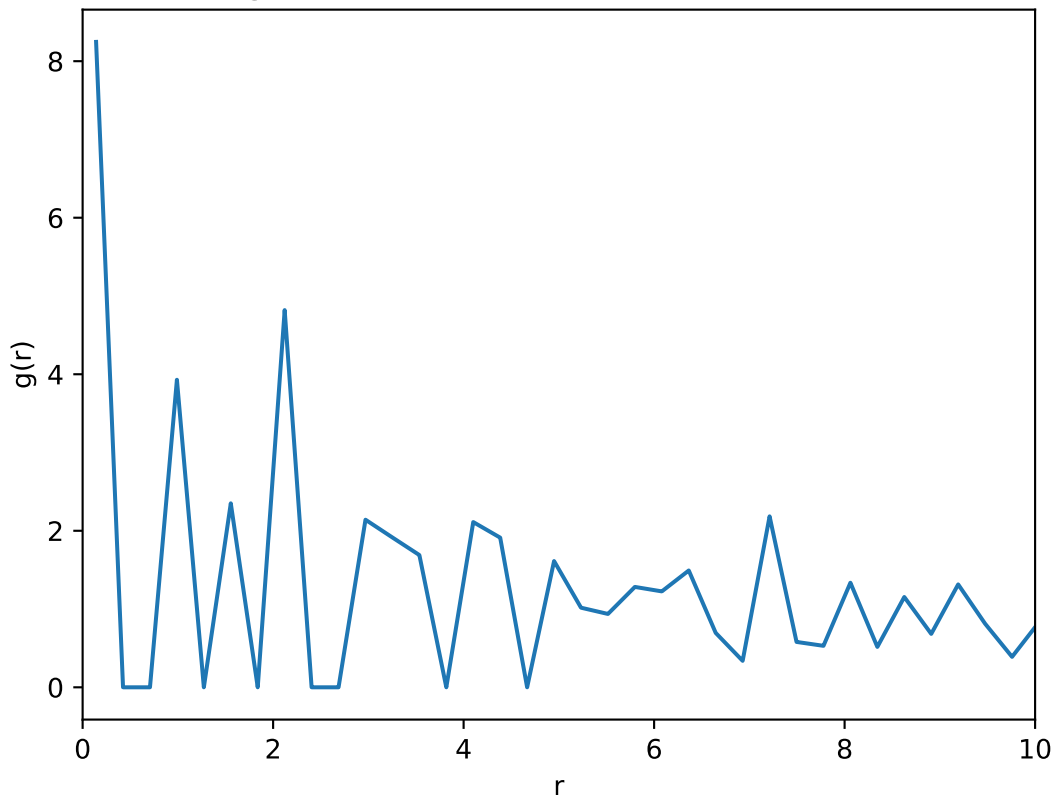
Average radial distribution function: T=0.52 , L=20
