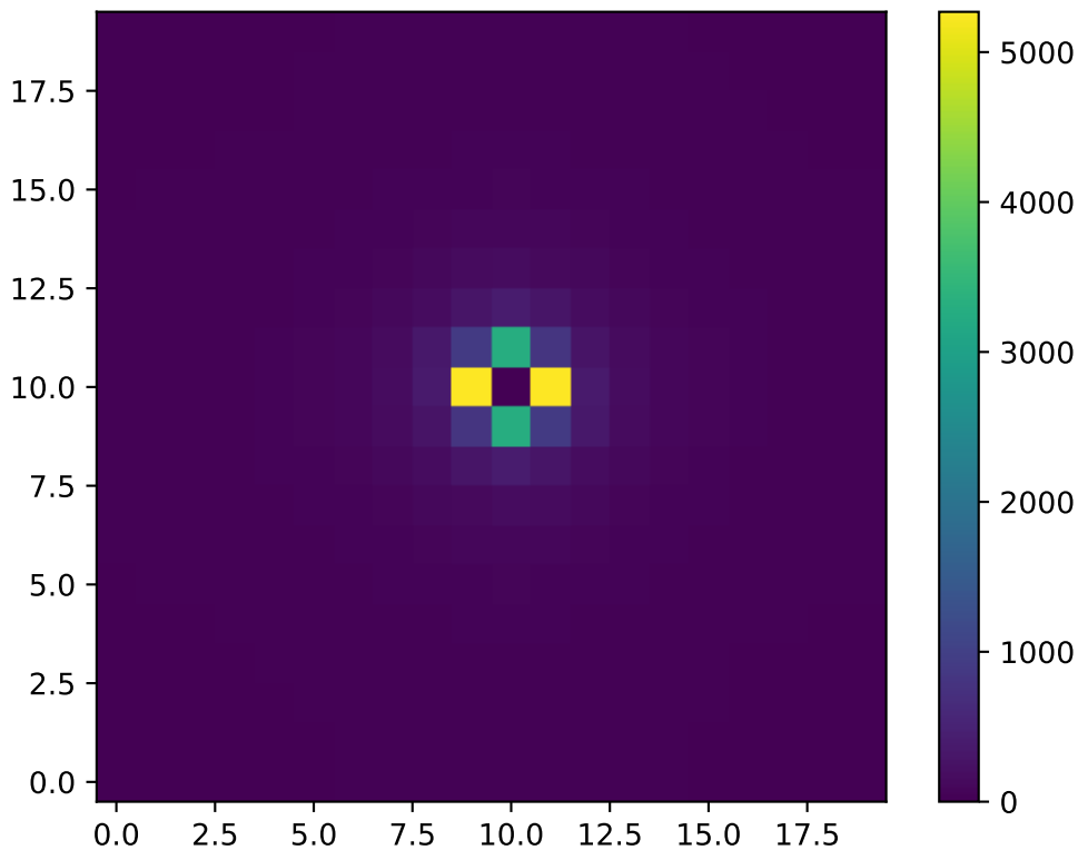
2D Structure Factor S(k) : T=0.52 , L=20
