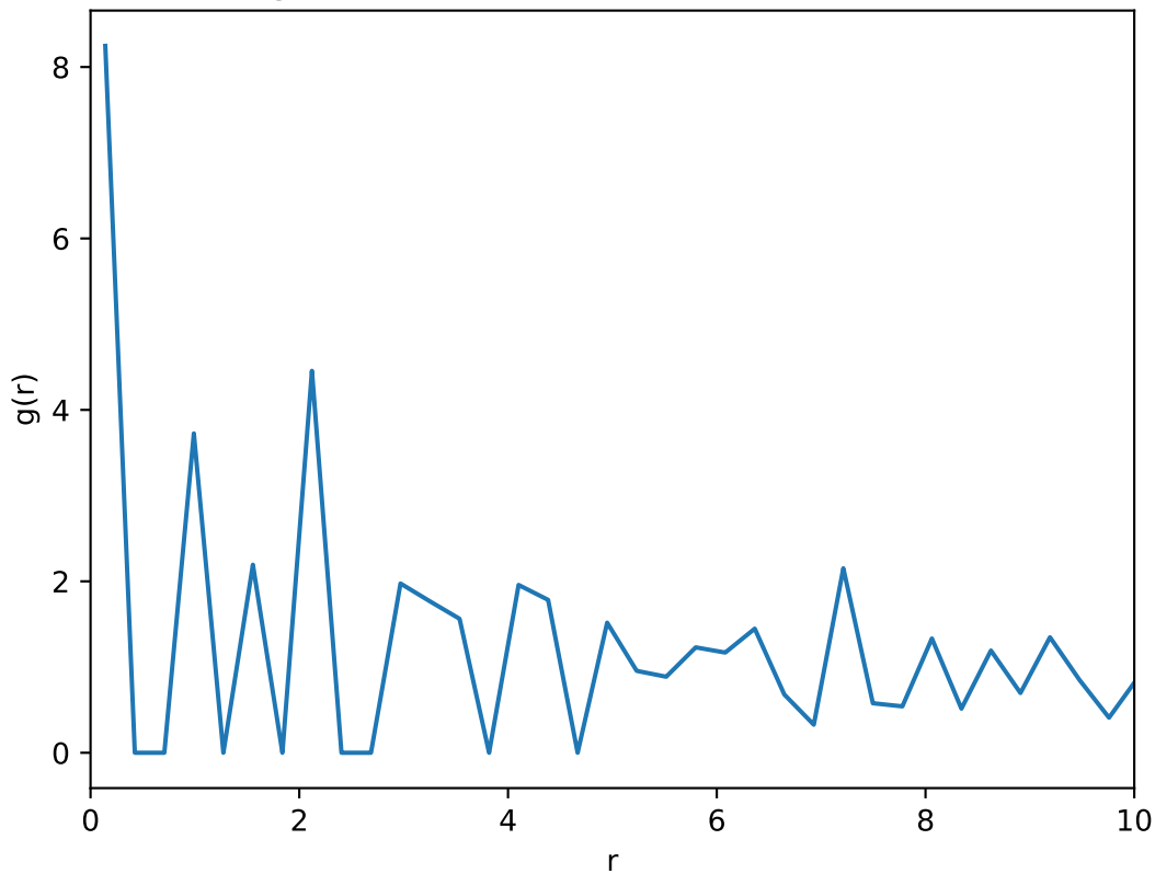
Average radial distribution function: T=0.57 , L=20
