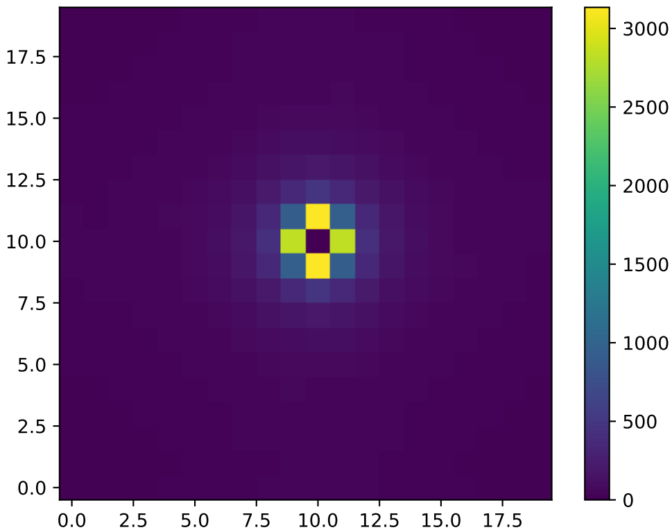
2D Structure Factor S(k) : T=0.57 , L=20
