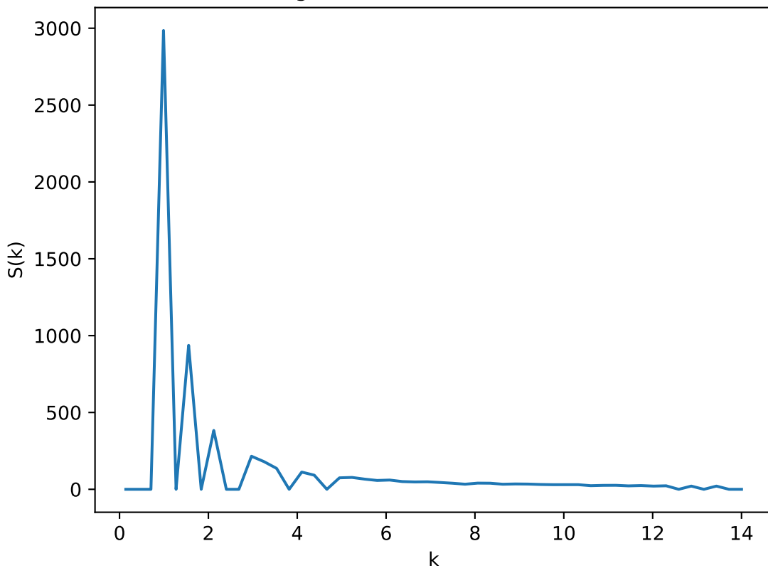
Radial Average of Structure Factor: T=0.57 , L=20
