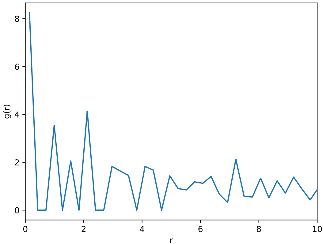
Average radial distribution function: T=0.63 , L=20
