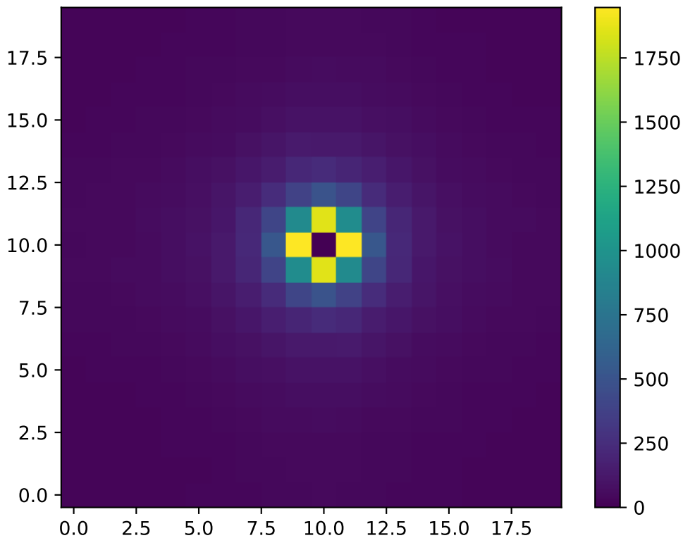
2D Structure Factor S(k) : T=0.63 , L=20
