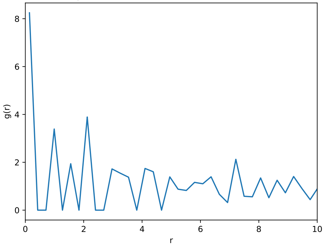
Average radial distribution function: T=0.68 , L=20
