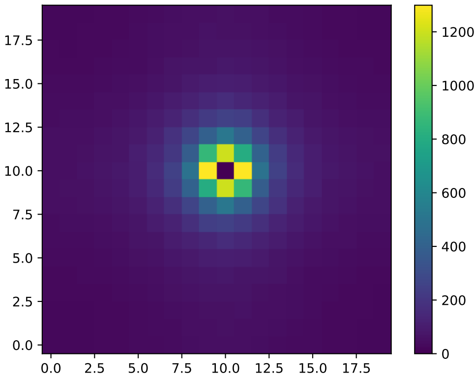
2D Structure Factor S(k) : T=0.68 , L=20
