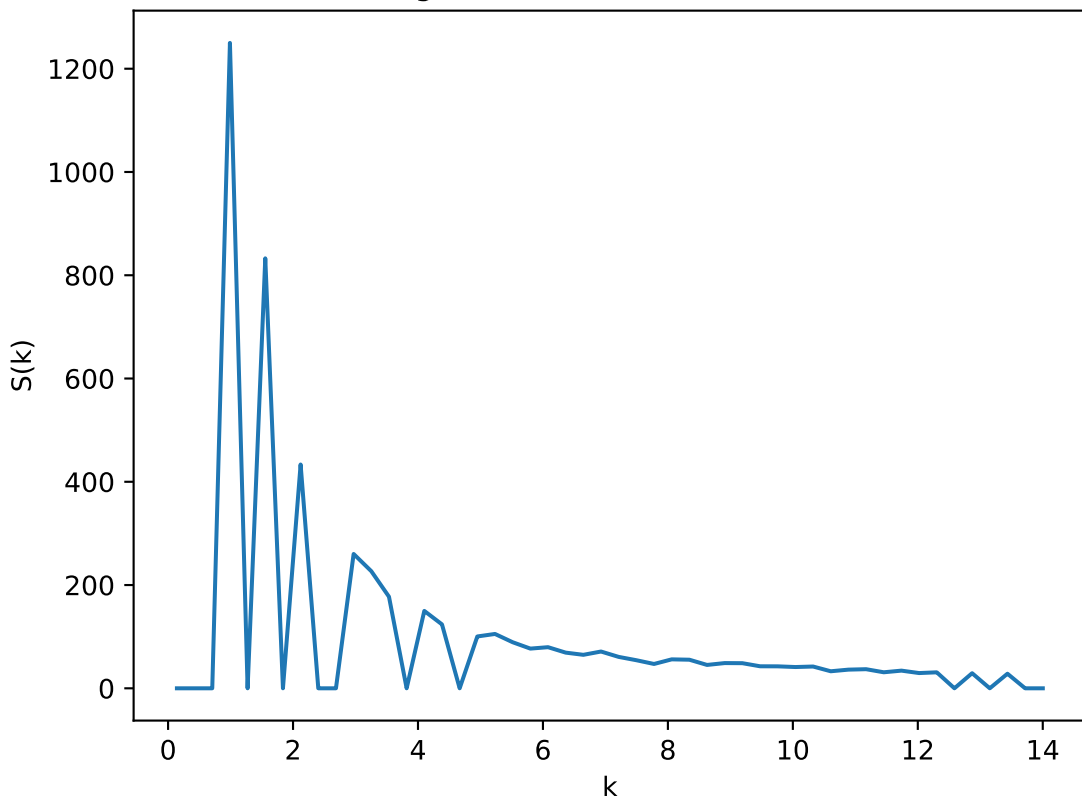
Radial Average of Structure Factor: T=0.68 , L=20
