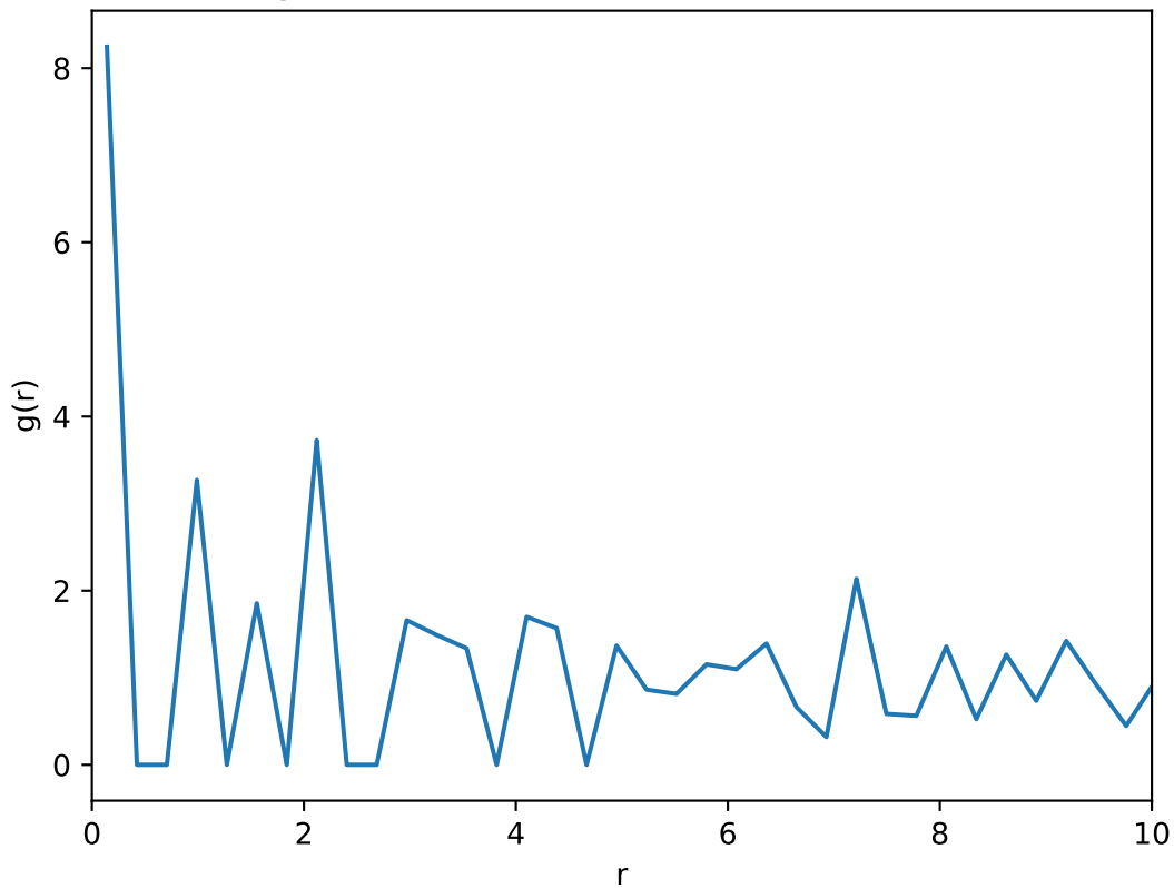
Average radial distribution function: T=0.74 , L=20
