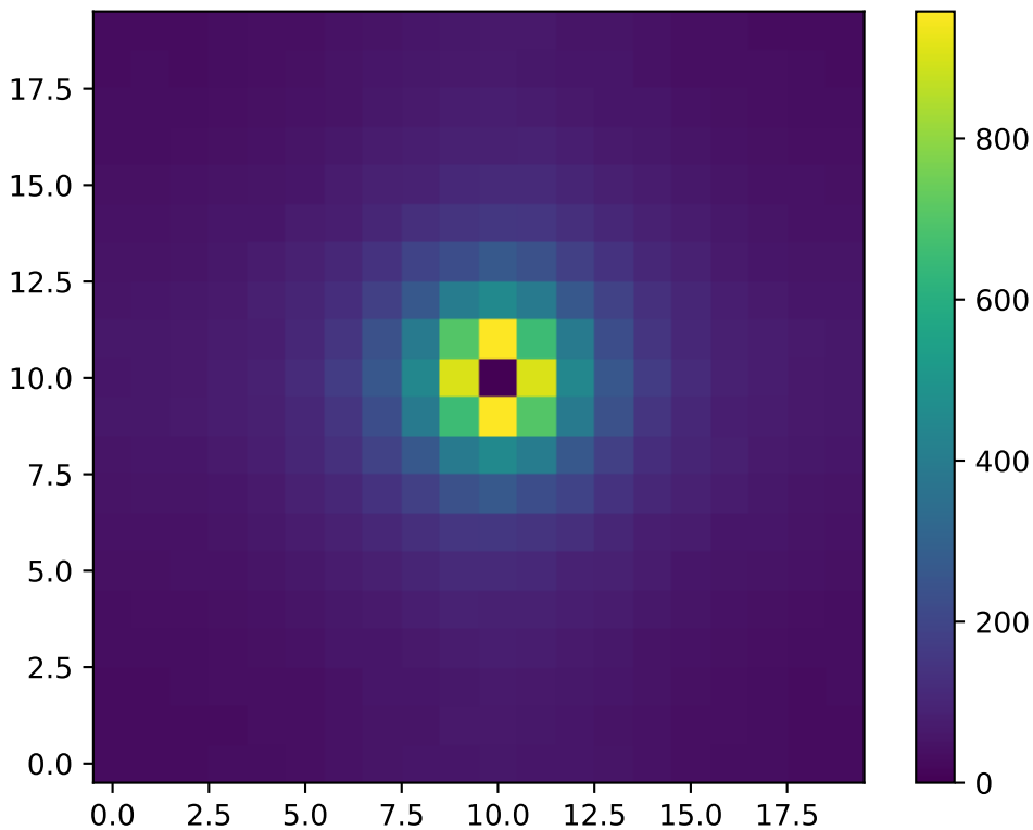
2D Structure Factor S(k) : T=0.74 , L=20
