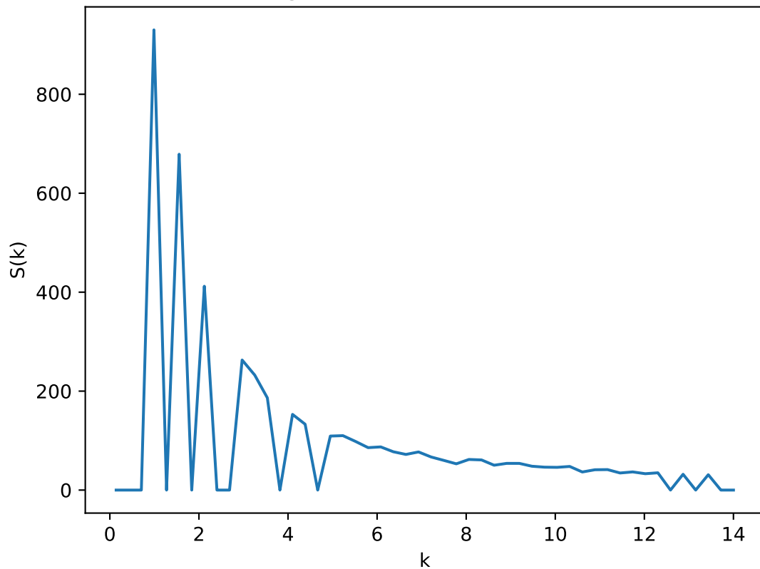
Radial Average of Structure Factor: T=0.74 , L=20
