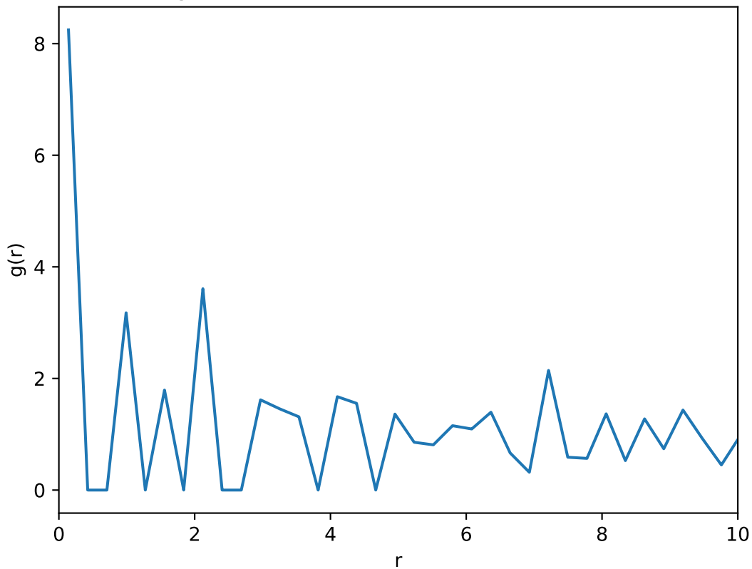
Average radial distribution function: T=0.79 , L=20
