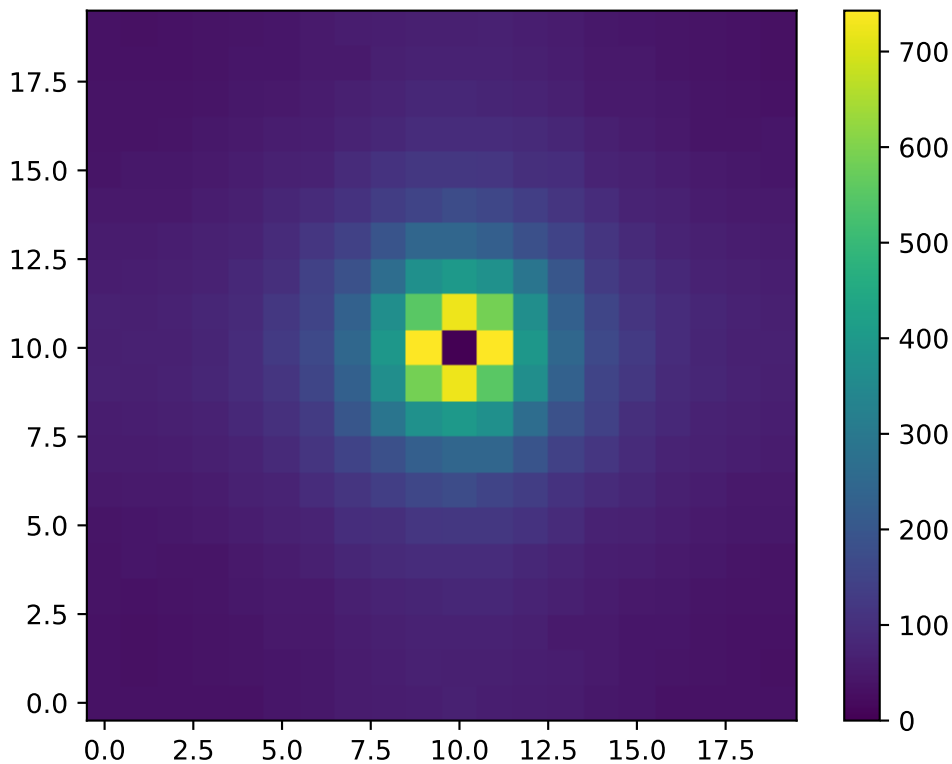
2D Structure Factor S(k) : T=0.79 , L=20
