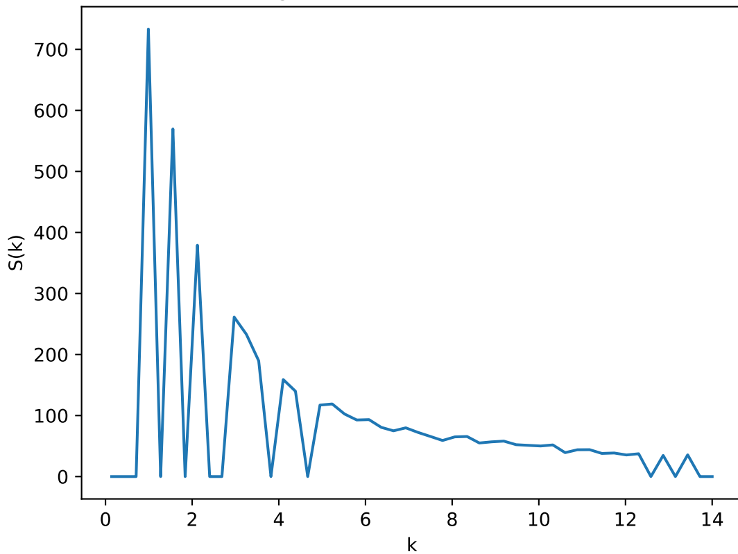
Radial Average of Structure Factor: T=0.79 , L=20
