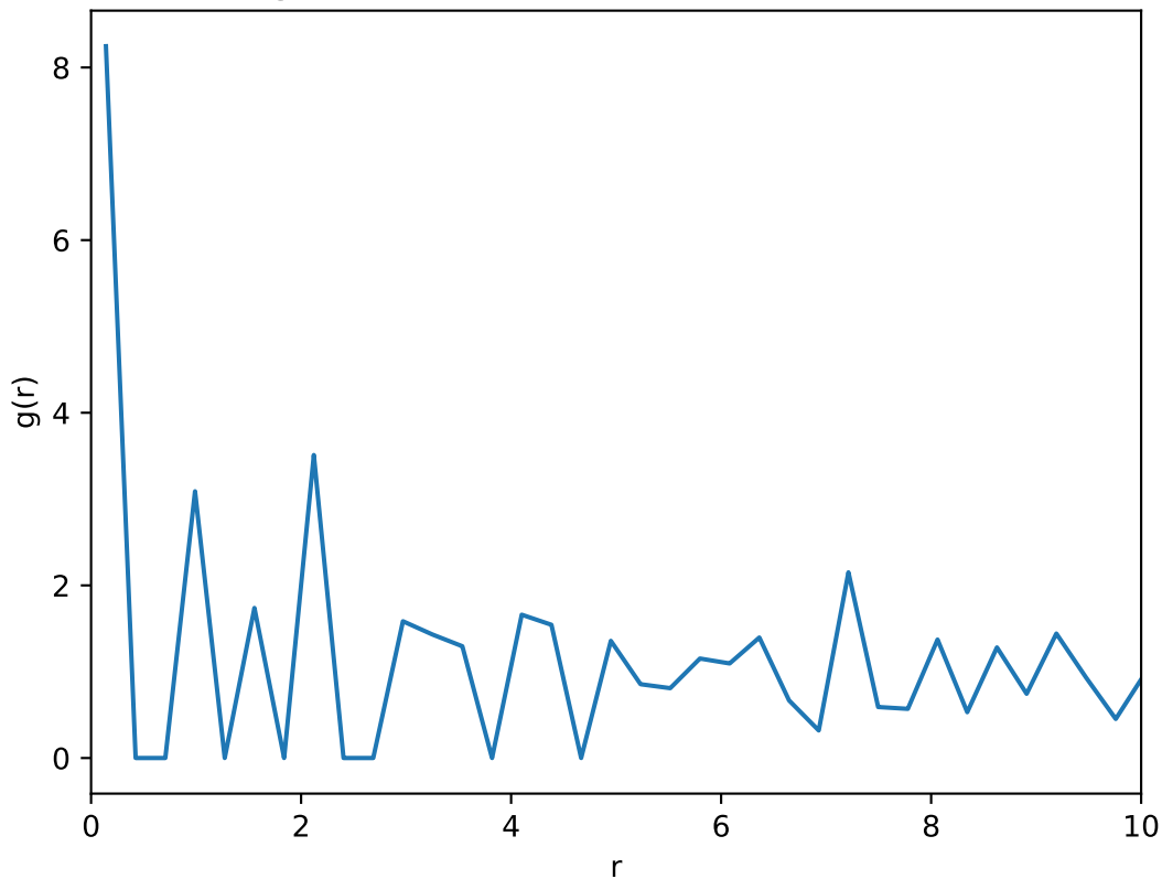
Average radial distribution function: T=0.85 , L=20
