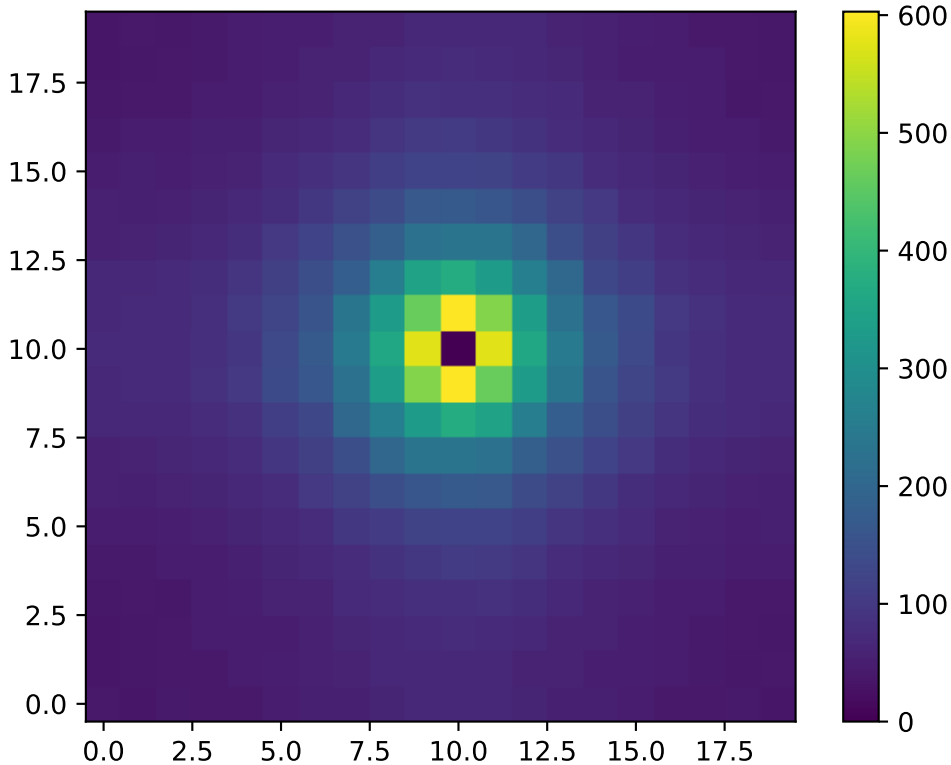
2D Structure Factor S(k) : T=0.85 , L=20
