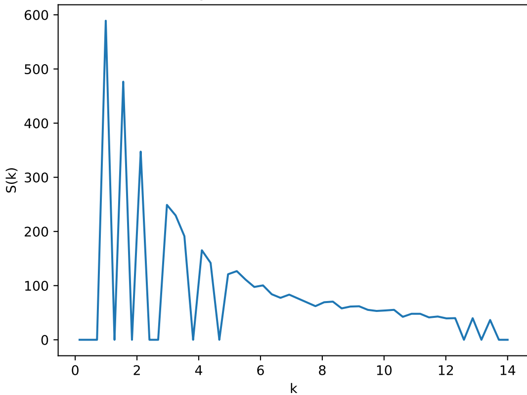
Radial Average of Structure Factor: T=0.85 , L=20
