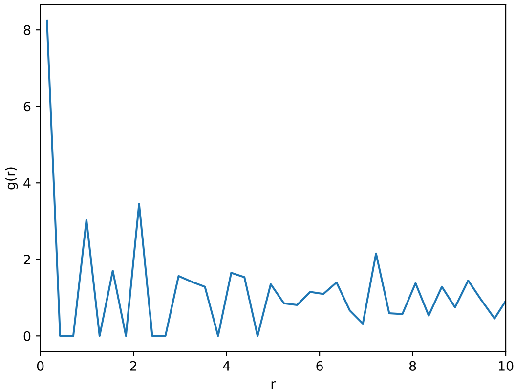
Average radial distribution function: T=0.90 , L=20
