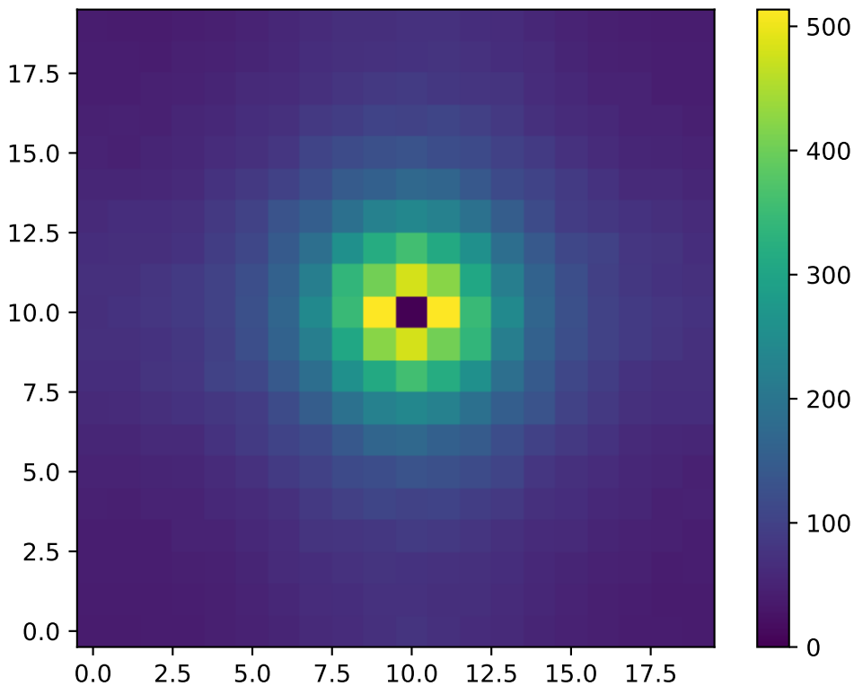
2D Structure Factor S(k) : T=0.90 , L=20
