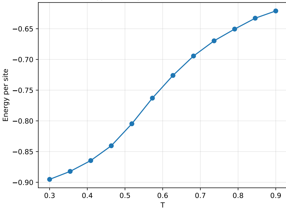
Energy vs Temperature ( L=20 , \rho=0.50 )
