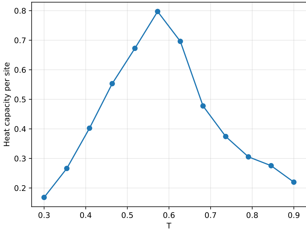
Heat Capacity vs Temperature ( L=20 , \rho=0.50 )
