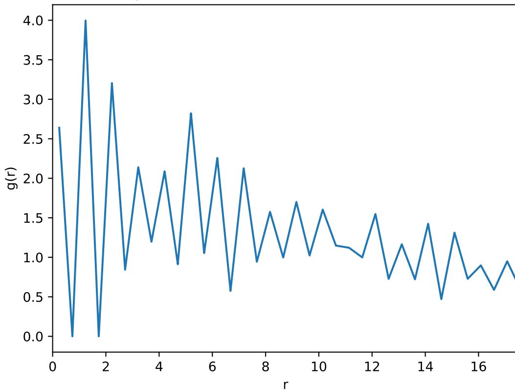
Average radial distribution function: T=0.30 , L=35
