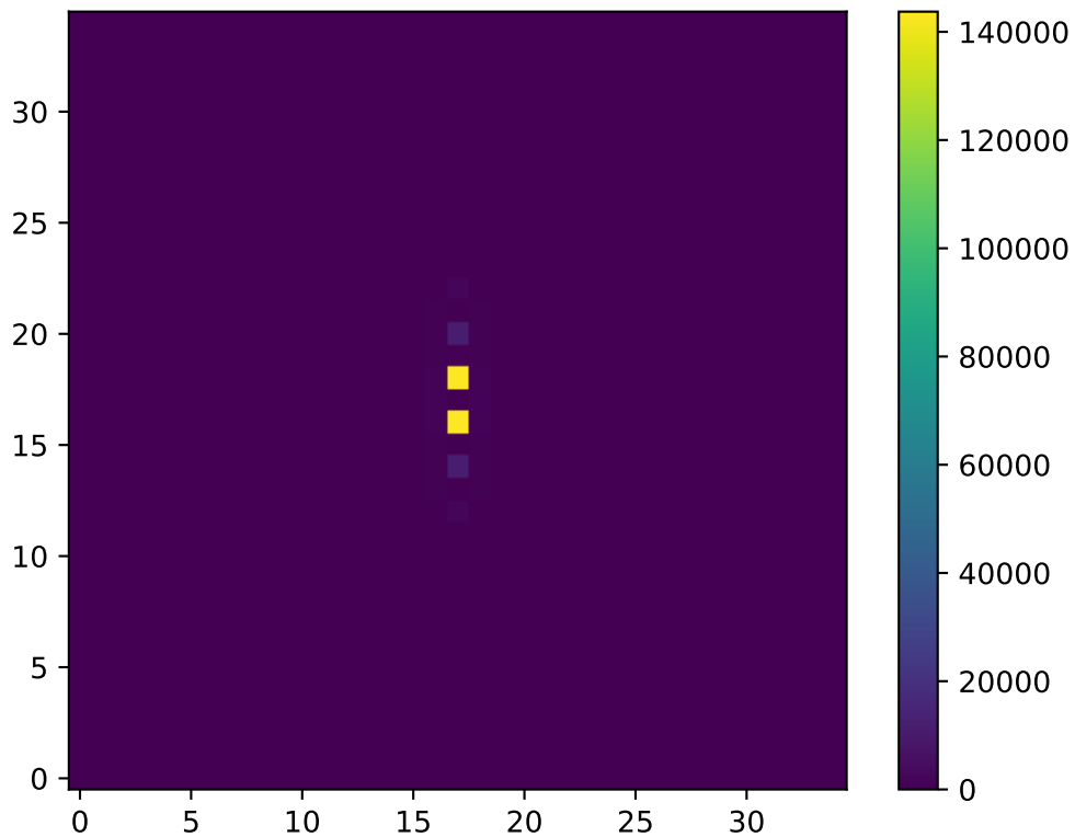
2D Structure Factor S(k) : T=0.30 , L=35
