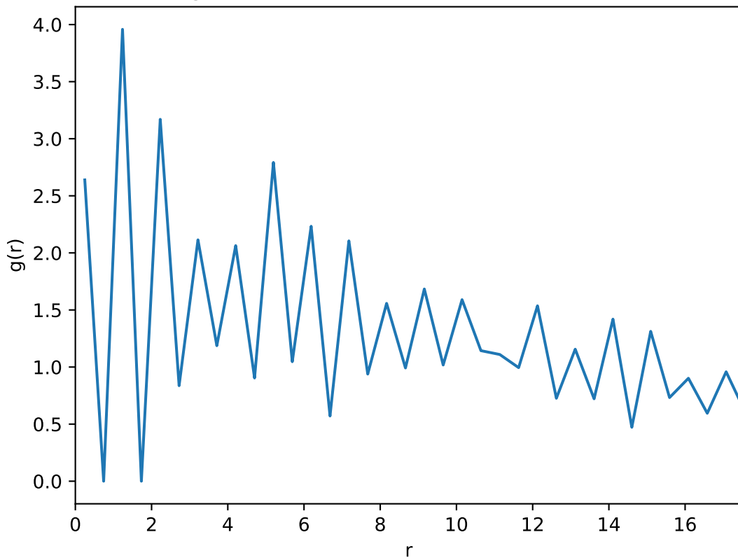
Average radial distribution function: T=0.35 , L=35
