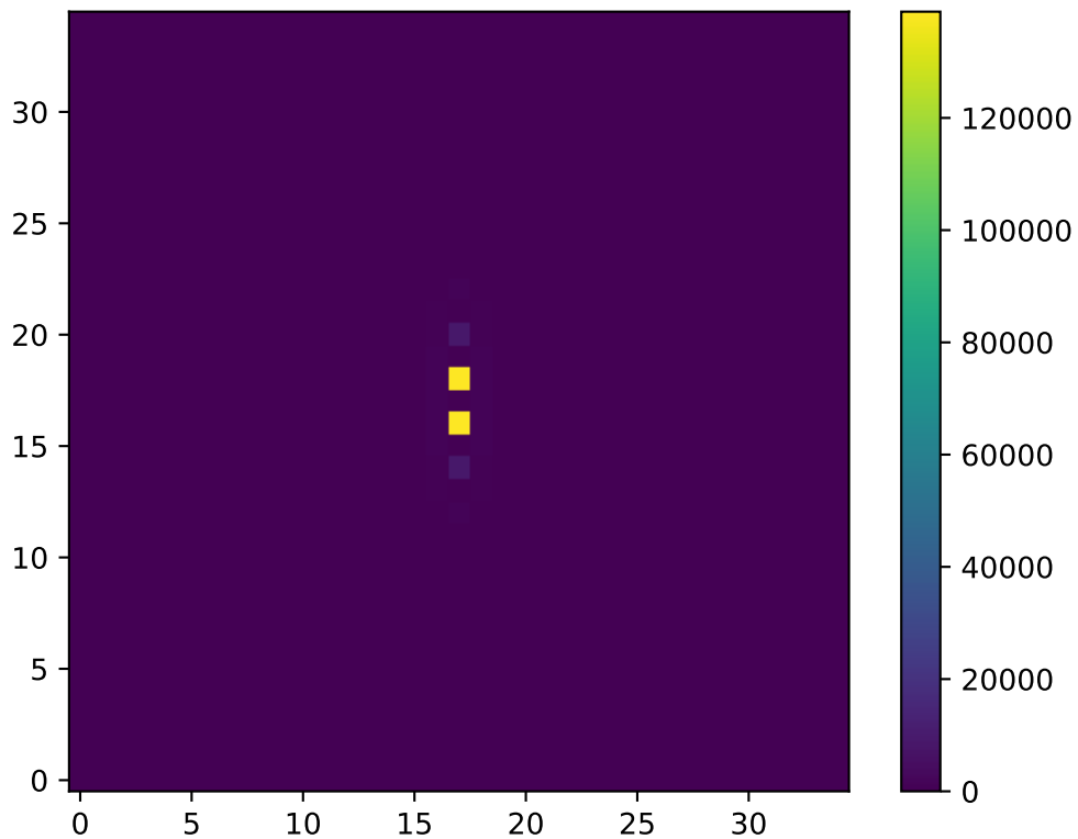
2D Structure Factor S(k) : T=0.35 , L=35
