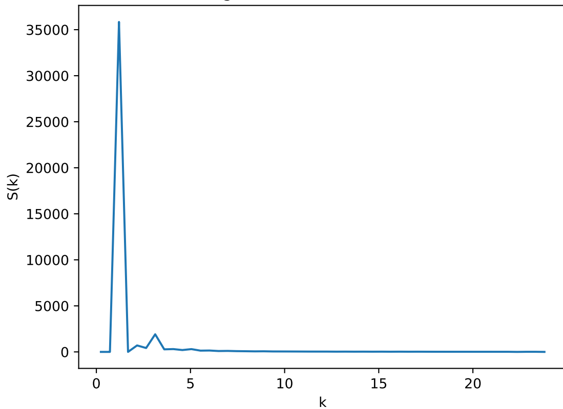
Radial Average of Structure Factor: T=0.35 , L=35
