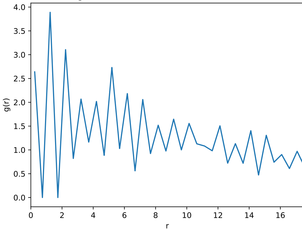
Average radial distribution function: T=0.41 , L=35
