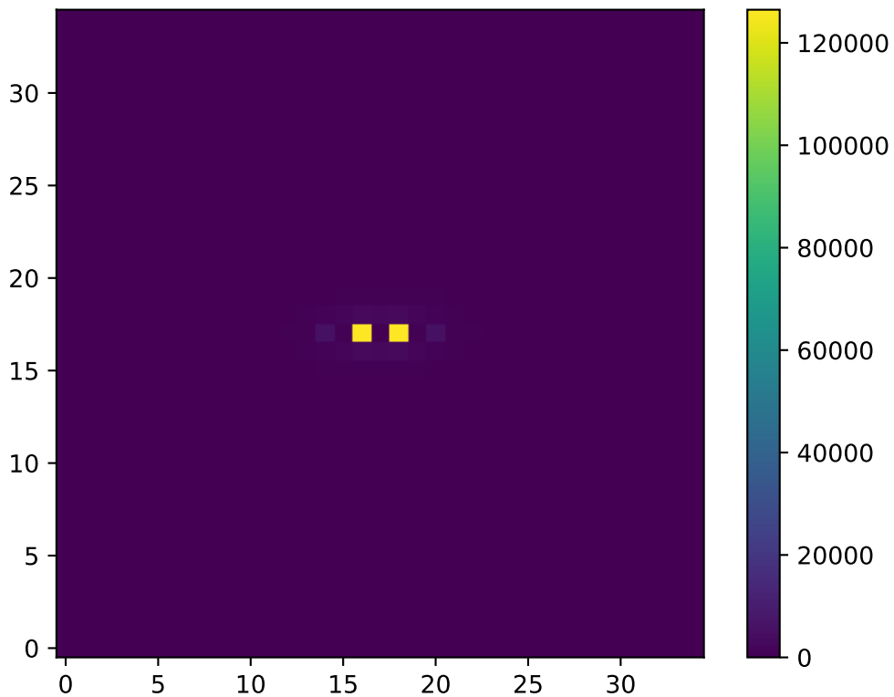
2D Structure Factor S(k) : T=0.41 , L=35
