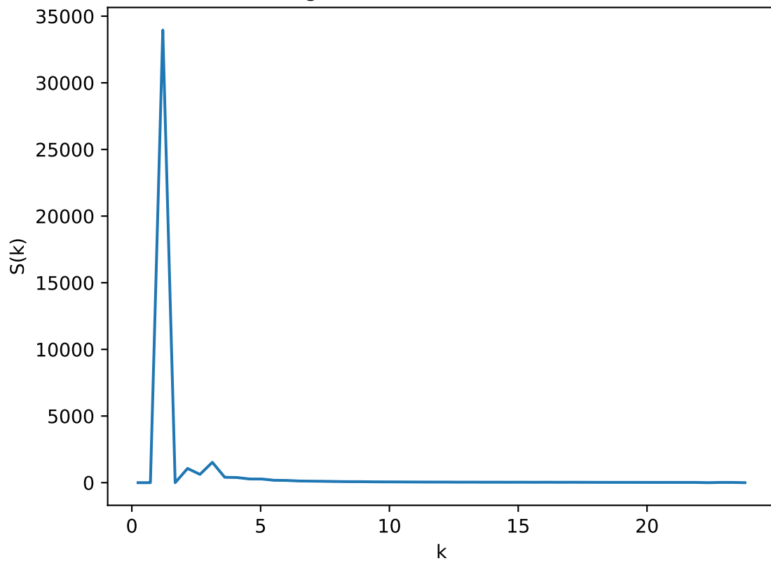
Radial Average of Structure Factor: T=0.41 , L=35
