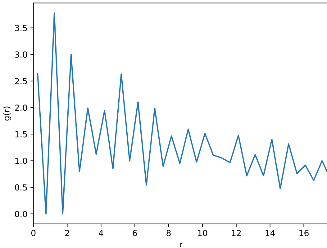
Average radial distribution function: T=0.46 , L=35
